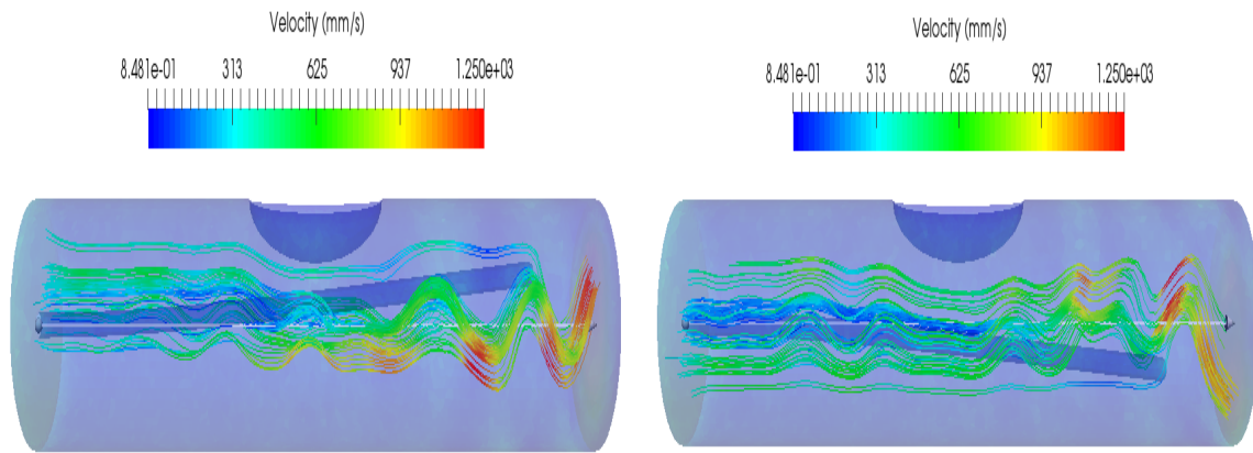
Figure 5.15: Left: velocity streamlines corresponding to sample 49: L = 3.712 , coef = 55.08 and FFR = 0.4043 . Right: velocity streamlines of sample 54: L = 3.86 , coef = -59.0136 and FFR = 0.38 .
