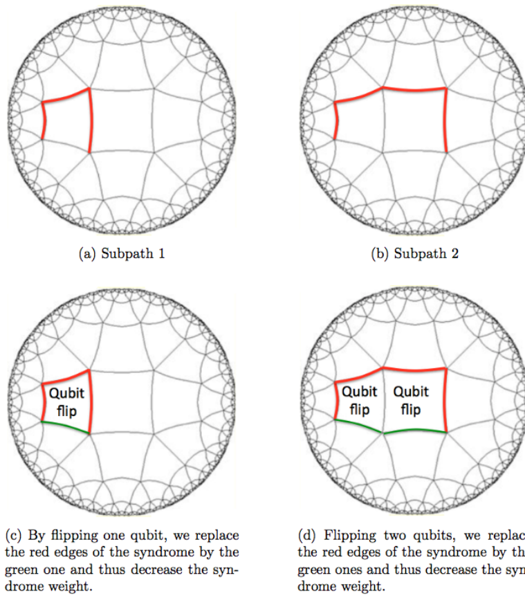
Figure 2.1: In the \{4, 5\} tessellation of hyperbolic plane, every loop of edges contains one of the two subpaths in red. These two subpaths are not minimal: they can be replaced by the shorter green ones by flipping one or two qubits. (source for image: [tes])
