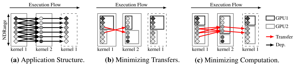
Figure 2.16: Impact on amount of data to transfer of different partitioning strategies.
