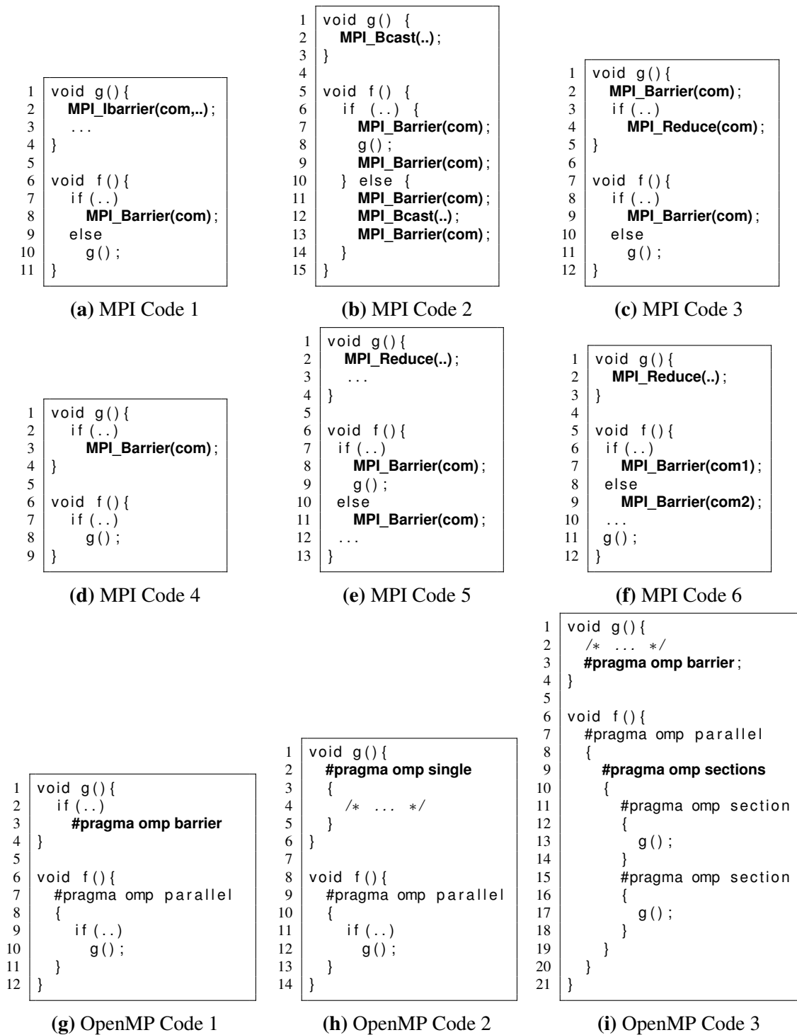
Figure 5.4: Examples of MPI and OpenMP codes.
