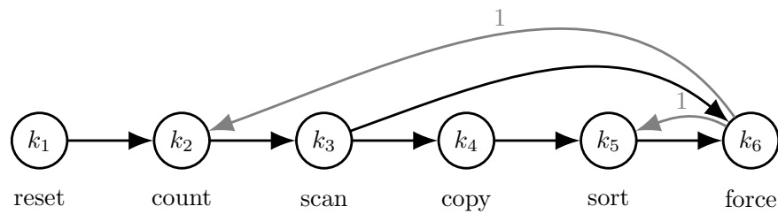
(a) Dependence graph between kernels.
