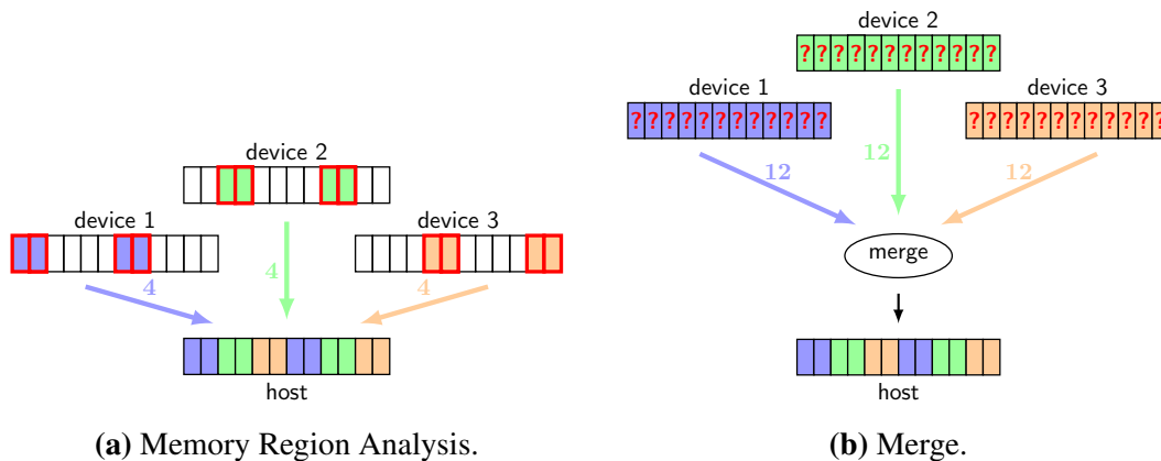
Figure 2.7: Partitioning Output Arrays. The partial region written by each device is highlighted in red. With a memory analysis only the partial regions written by each device are transferred to the host.
