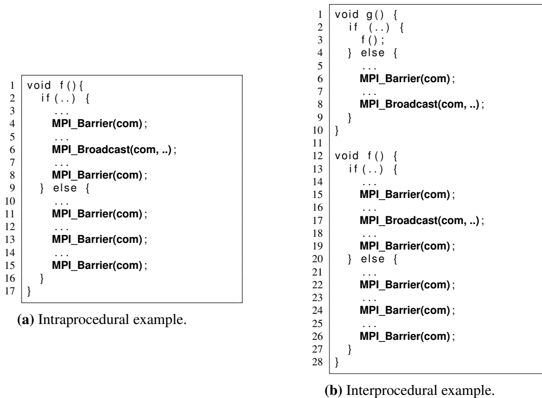
Figure 5.1: MPI examples of control-flow divergences that may lead to the execution of different sequences of collectives by different processes.
