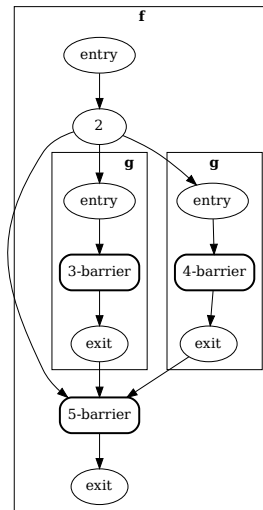
(a) OpenMP code 3 PPCFG.
