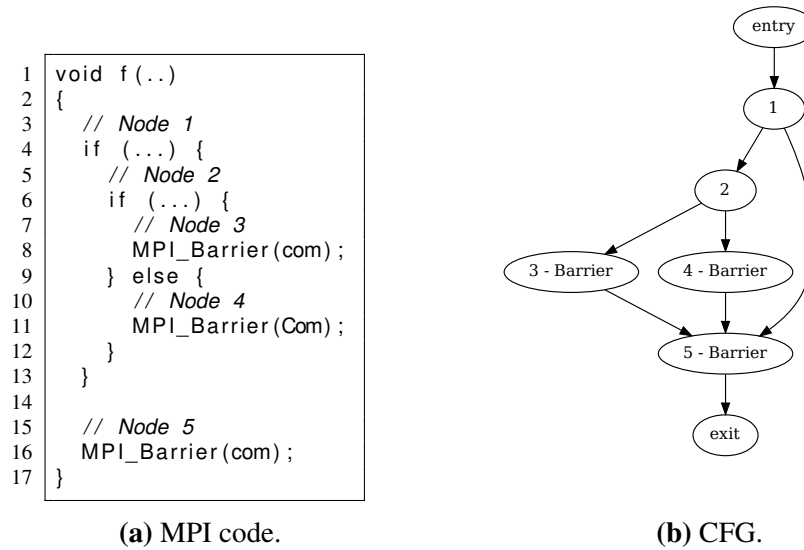
Figure 5.2: Example of Control Flow Graph.
