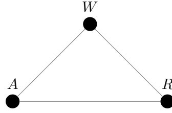
Figure 6.2: Graphical representation of log-linear model in Eq. 6.4.
