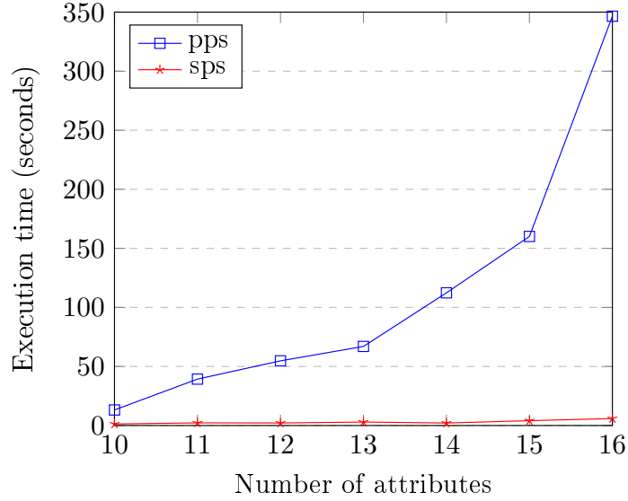
Figure 3.6: Comparison of partition pattern structure (pps) and sequence pattern structure (sps) in the task of finding OP biclusters in matrices with 10 rows and varying number of columns.
