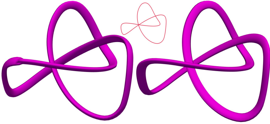
Figure 5.19: Convolution surface around a circular spline approximation of the knot \Gamma(t) = (-10\cos t - 2\cos 5t + 15\sin 2t, -15\cos 2t + 10\sin t - 2\sin 5t, 10\cos 3t) , t \in [0, 2\pi] . Anisotropic convolution parameters: \alpha_0 = \alpha_1 = \gamma_0 = \gamma_1 = 1 , \beta_0 = \beta_1 = 1/4 . On the left the surface without rotation: \theta_0 = \theta_1 = 0 , on the right the surface with a corrective rotation: \theta_0 = 0 and \theta_1 = -1.89 . In the middle we show the skeleton. We used 19 biarcs to approximate \Gamma .
