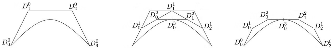
Figure 3.2 – Steps of the de Casteljau algorithm applied to a Bézier curve of degree 3 along with the induced subdivision in two.
