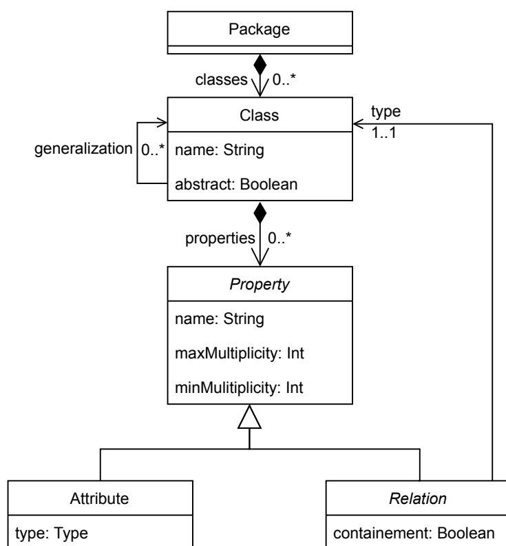
Figure 2.2 – Extract of self-descriptive meta-metamodel.
