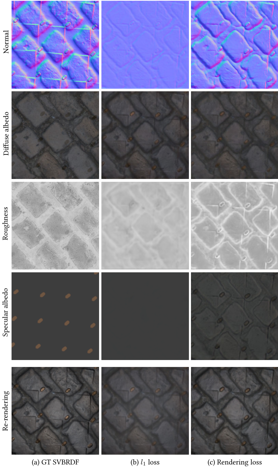
Figure 3.6: When trained with the l_1 loss (b), the SVBRDF predicted by the network for a test input image does not accurately reproduce the appearance of the target material when rendered. A network trained using the rendering loss (c) produces an SVBRDF
