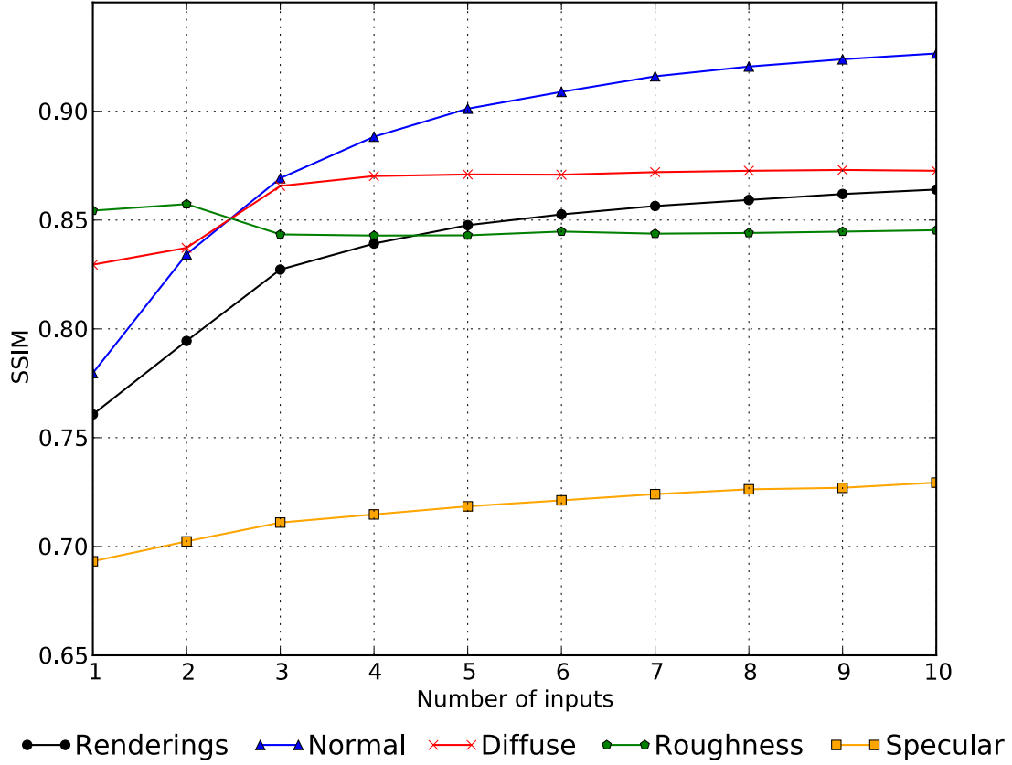
Figure 4.4: SSIM of our predictions with respect to the number of input images, averaged over our synthetic test dataset. The SSIM of re-renderings increases quickly for the first images, before stabilizing at around 10 images. The normal maps strongly benefit from new images. Diffuse and specular albedos also improve with additional inputs, which is not the case of the roughness that remains stable overall. We provide similar RMSE plots as supplemental materials.
