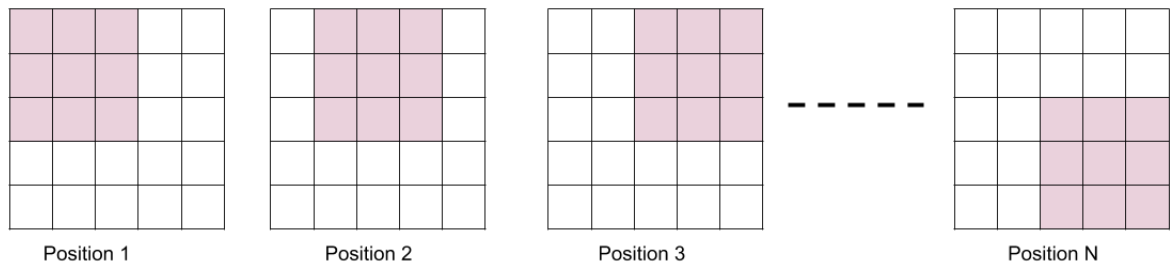
Different positions of a convolutional filter kernel as it slides over a feature map. For simplicity, here the feature map is of shape 5x5 and the filter kernel is of shape 3x3.
