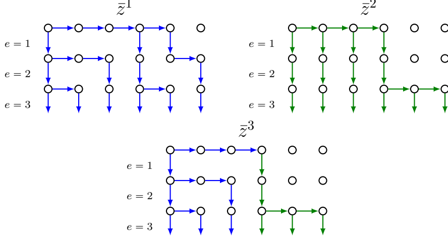
Figure 2.3: Two decision trees associated with subproblem solutions \bar{z}^1 and \bar{z}^2 . Their recombination \bar{z}^3 is feasible for [R'_{LP}] , but not feasible for [M'_{LP}] , both defined by the same subset P' \supseteq \{1, 2\} of solutions.
