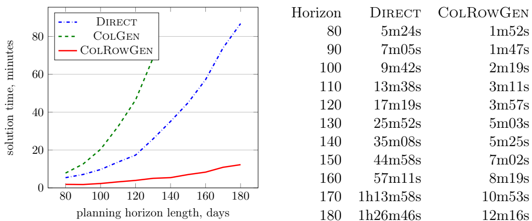
Figure 3.2: Solution times for test instances with larger planning horizon length
