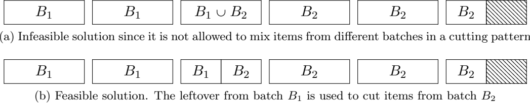
Figure 3.5: Representation of a solution for two batches B_1 and B_2 .
