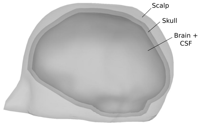
Figure 2.1: Example of a piecewise homogeneous conductor model of the head. Three layers are used: Scalp, skull and brain and cerebrospinal fluid (CSF).
