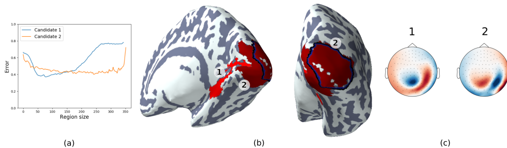
Figure 6.10: Source 2. (a) Candidate projection error as a function of a region size. (b) Candidate upper bound regions on the cortex (shades of red) and simulated region (dark border). (c) Topographies associated to the best nodes of candidate growing regions.
