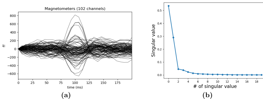
Figure 6.1: (a) Simulated MEG signal with additive noise (b) Squares of the singular values of the normalized signal.
