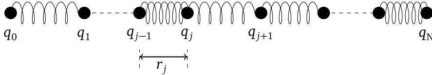
Figure 2.1: One-dimensional coupled oscillators.
