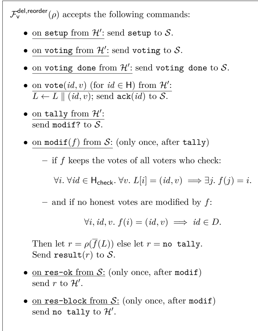
Figure 6.8: The ideal functionality \mathcal{F}_v^{\text{del, reorder}}(\rho) .
