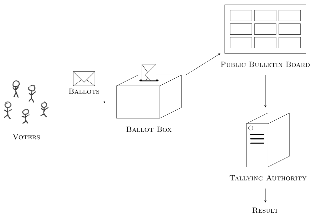
Figure 1: The Helios voting protocol
