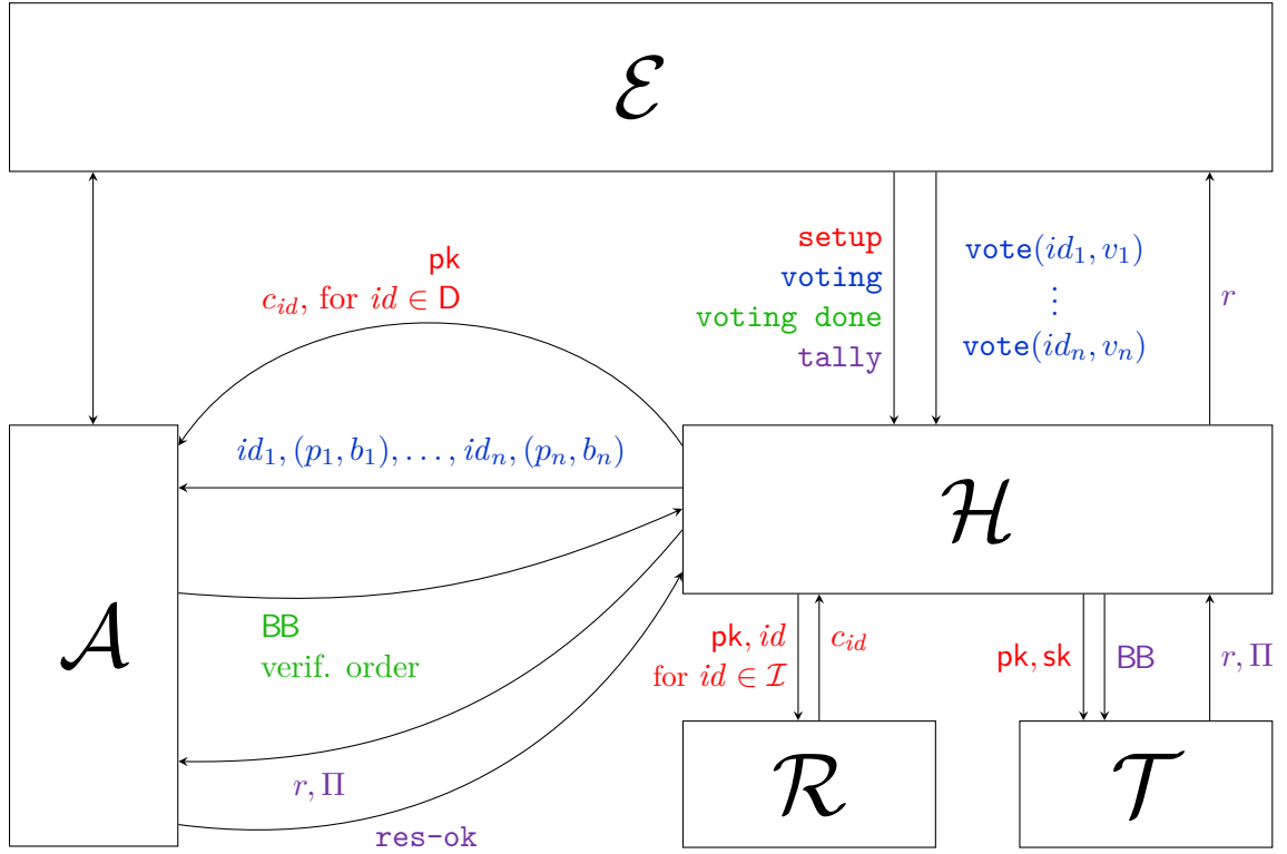
Figure 6.6: The real execution with id_1, \dots, id_n \in \mathcal{H}
