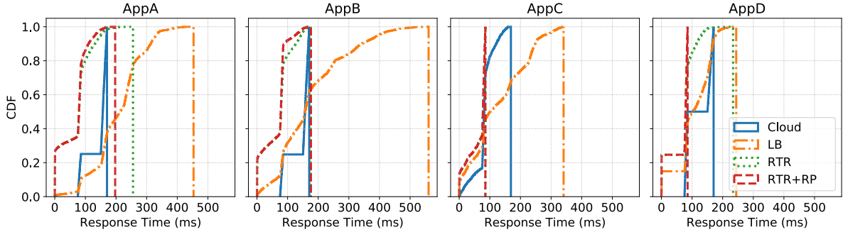
Figure 4.6: CDF of response times for complex applications.
