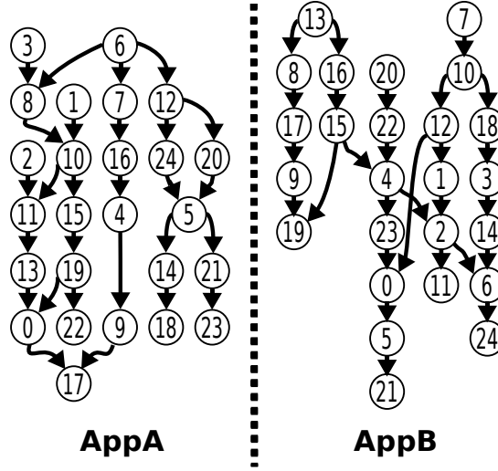
Figure 5.2: Evaluated applications.
