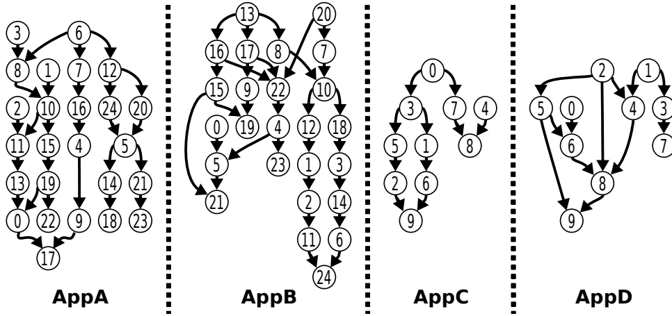
Figure 4.4: Complex applications.
