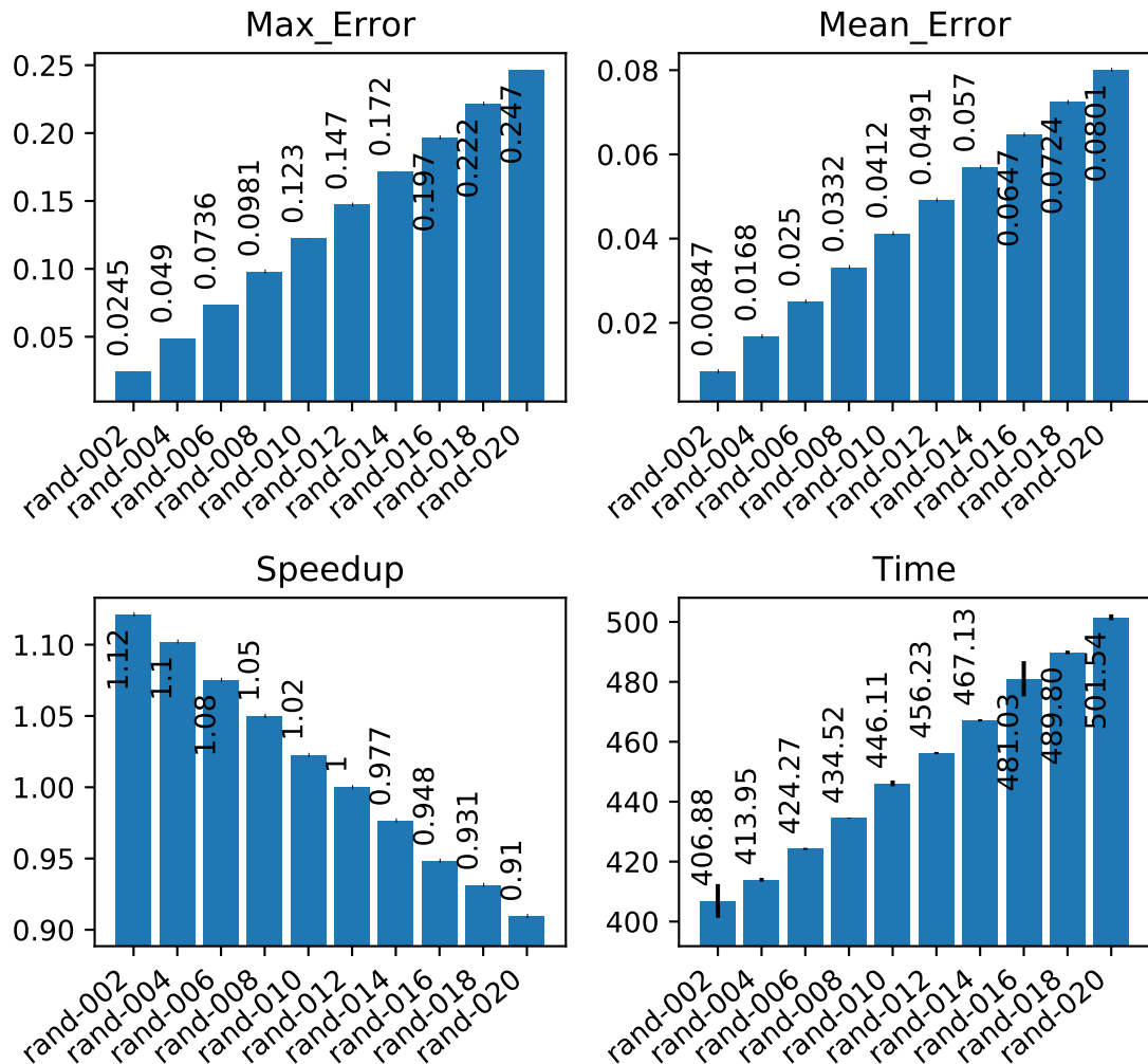
Figure 7.1 – LetItBench Generated Plot Plot generated from LetItBench space-separated CSV data. In this example, some computation of the heatsolve application (Section 7.1.3) are skipped randomly with a probability expressed in percentage and appended to the name of the benchmark run . Five executions of each run have been executed to generate this plot with error bars. The speedup can optionally be computed by the script, here we selected the Time data with the base value rand-012.
