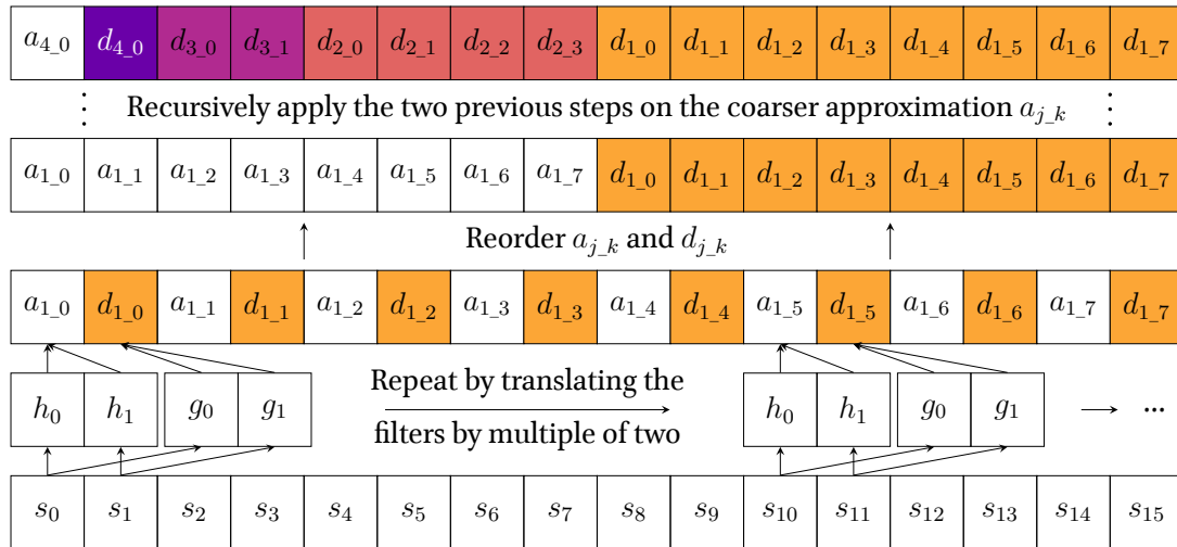
Figure 6.3 – Discrete Wavelet Transform The wavelet decomposition of an evenly sampled signal (s_i) with filters of size 2. The algorithm consists of an application of filters h and g which respectively compute a coarser approximation (a_{j,k}) and the details lost by applying h (d_{j,k}) at the level j and a translation of 2k . This step is usually followed by packing the coarser approximation and details together. These two steps are applied recursively until the number of remaining coarse approximation (a_{j,k}) is lower than the size of a filter.
