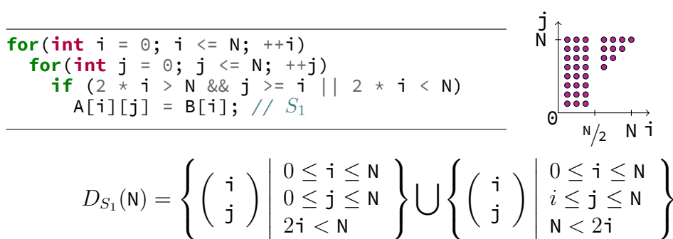
Figure 2.5 – Polyhedral Model Representations of Codes Multiple abstract representation of a same iteration domain. The source code in the C language is represented at the top-left. The iteration domain is represented in the polyhedral model by a union of two sets of inequation shown at the bottom. The resulting parametrized polyhedron is pictures at the top-right. Each point of the polyhedron represents an instance of the statement S_1 and its coordinates are the values taken by the induction variables (i, j) .
