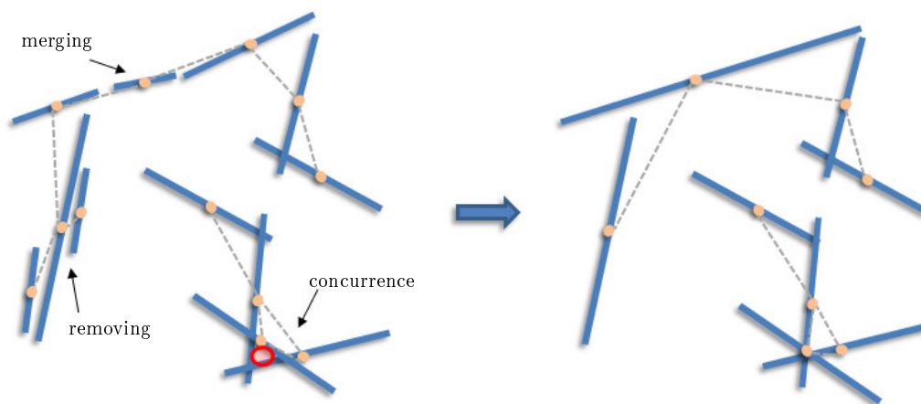
Figure 2.3: Line-segment consolidation. Three different operations applied greedily over the adjacency graph (dashed grey lines) bring spatial coherence between the detected line-segments. Such a consolidation procedure also reduces the problem complexity as the number of line-segments becomes lower.
