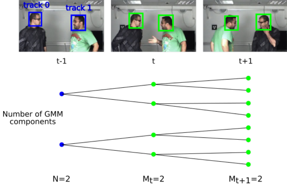
Figure 2.1: Illustration of growing number of GMM components in p(\mathbf{s}_t | \mathbf{o}_{1:t}) with EM solution. Green: detections; Blue: tracked person-state. Assume at t - 1 there are two tracked person and each of them follows a Gaussian distribution. Then at t + 1 the number of the GMM components in the filtering distribution p(\mathbf{s}_t | \mathbf{o}_{1:t}) will be N \times M_t \times M_{t+1} = 8 .
