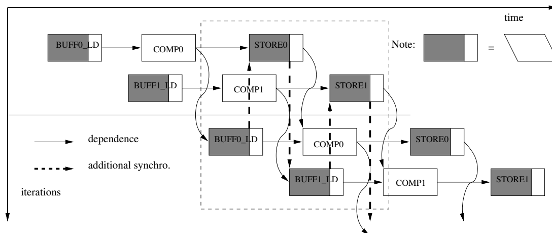
Figure 4.5 – Software pipeline
