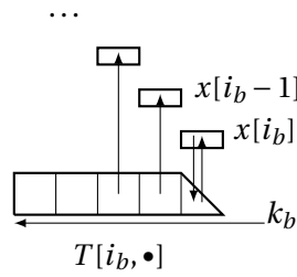
Figure 2.13 – Dependences between the tiles of T and the tiles of x/temp
