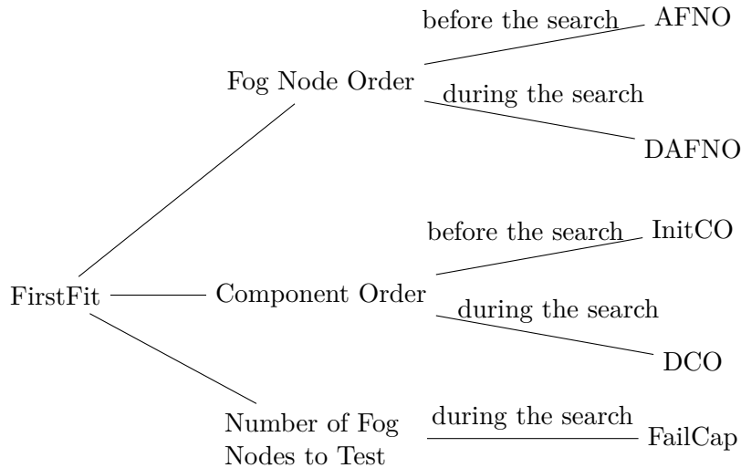
Figure 4.10: Heuristics Positioning.
