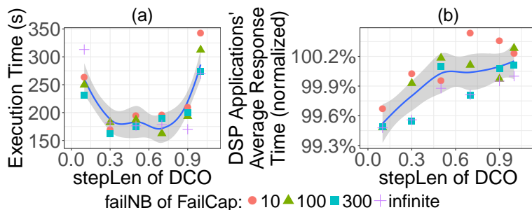
Figure 5.14: Evaluation Results with Different Parameters 13 .
