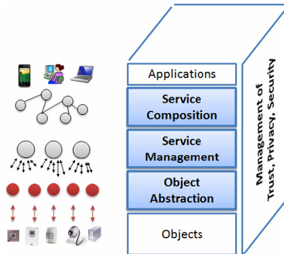
Figure 2.3: Middleware Architecture.
