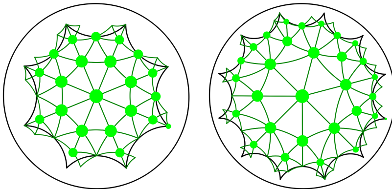
Figure V.18: Triangulations of \mathbb{M}_3 for g = 2 (left) and g = 3 (right) with dummy points generated with the sequential strategy.
