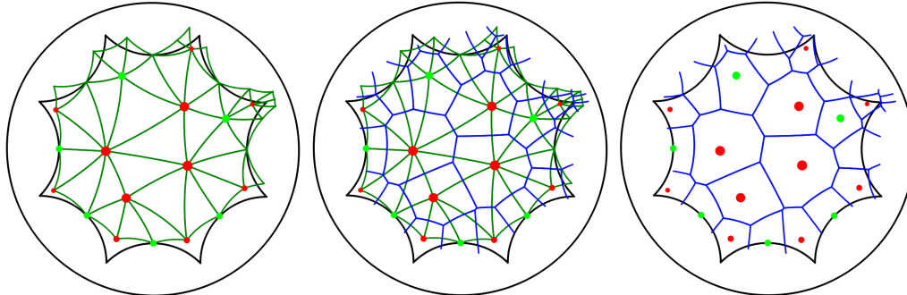
Figure IV.15: The figure shows a Delaunay triangulation with both dummy points and input points (left), the same Delaunay triangulation with the dual objects of its faces and edges (center), and just the dual objects of the Delaunay triangulation (right).
