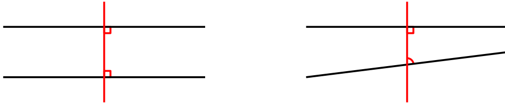
Figure II.1: Illustration of the fifth postulate of Euclid. Given two lines and a third one incident to both, if the sum of the internal angles on one side is two right angles (left), then the lines are parallel. If the sum of the internal angles on one side is less than two right angles (right), then the lines intersect on that side.
