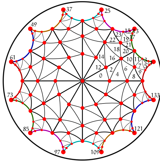
Figure V.15: Initialization of DT_{\mathbb{M}_g}(Q_g) with deterministic set of dummy points. The number next to each vertex is the identifier of the face incident to that vertex.
