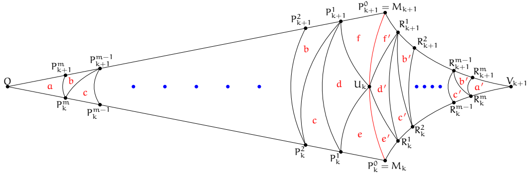
Figure V.14: Zoom on the faces of the triangulation of \mathbb{M}_g defined by the deterministic dummy points.
