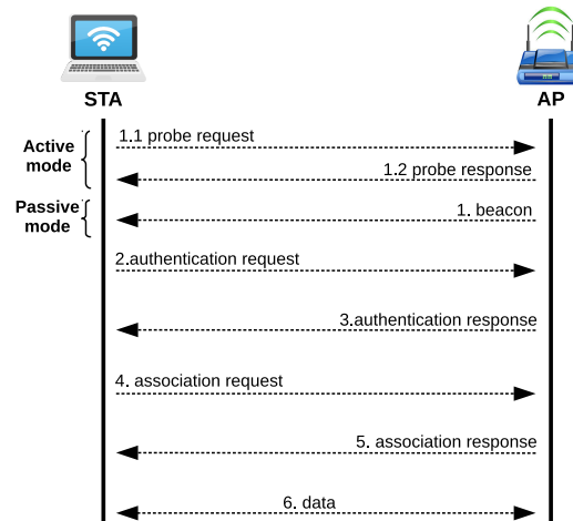
Figure 1.5: Association process.
