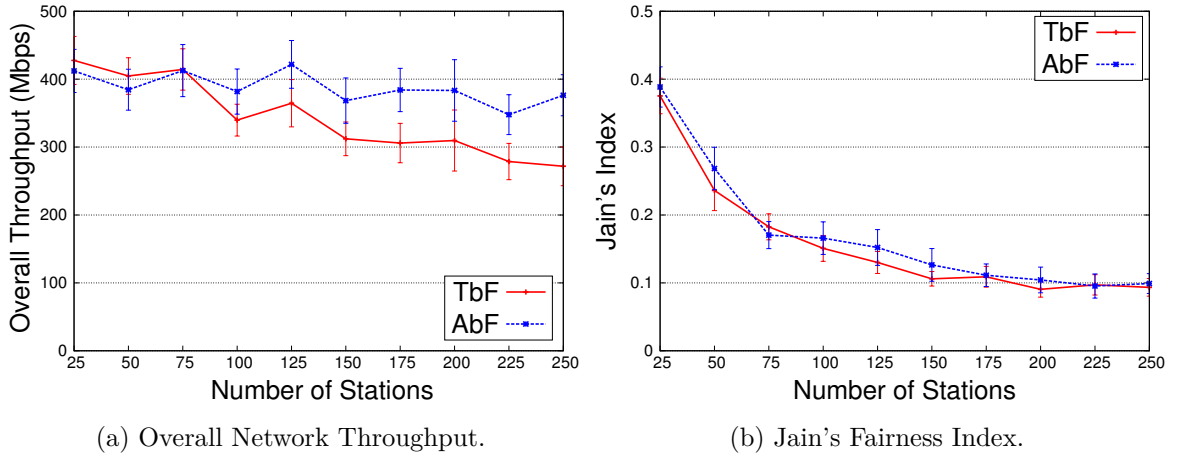
Figure 3.13: 3 Orthogonal Channels
