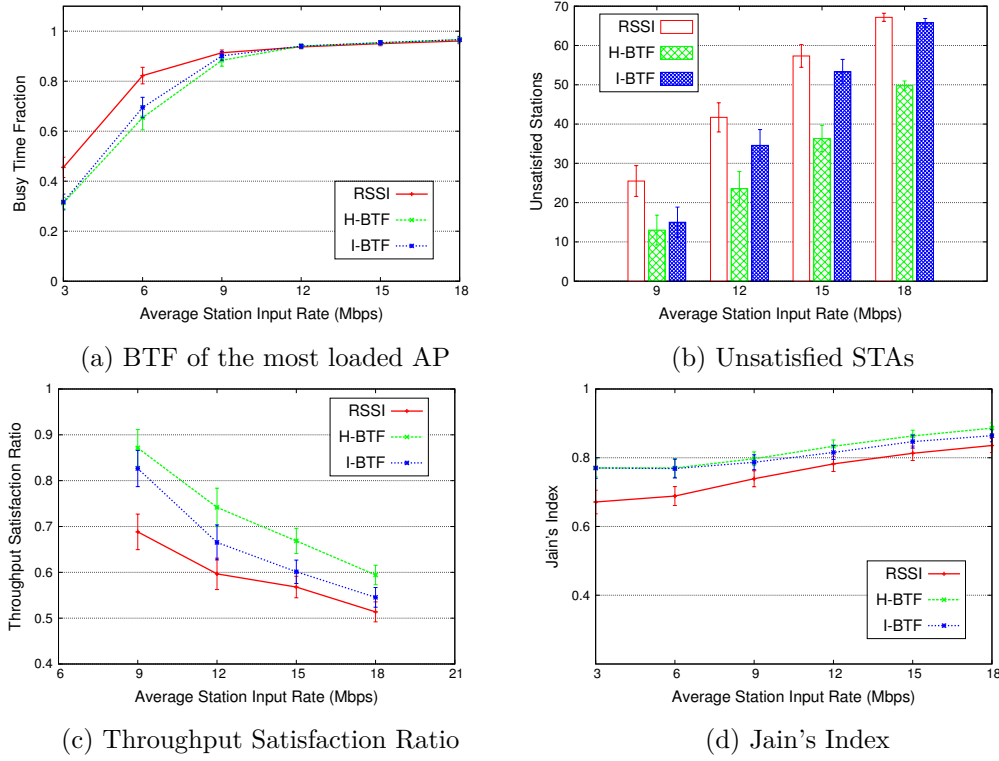
Figure 5.4: BTF association optimization using the random topology with TCP flows
