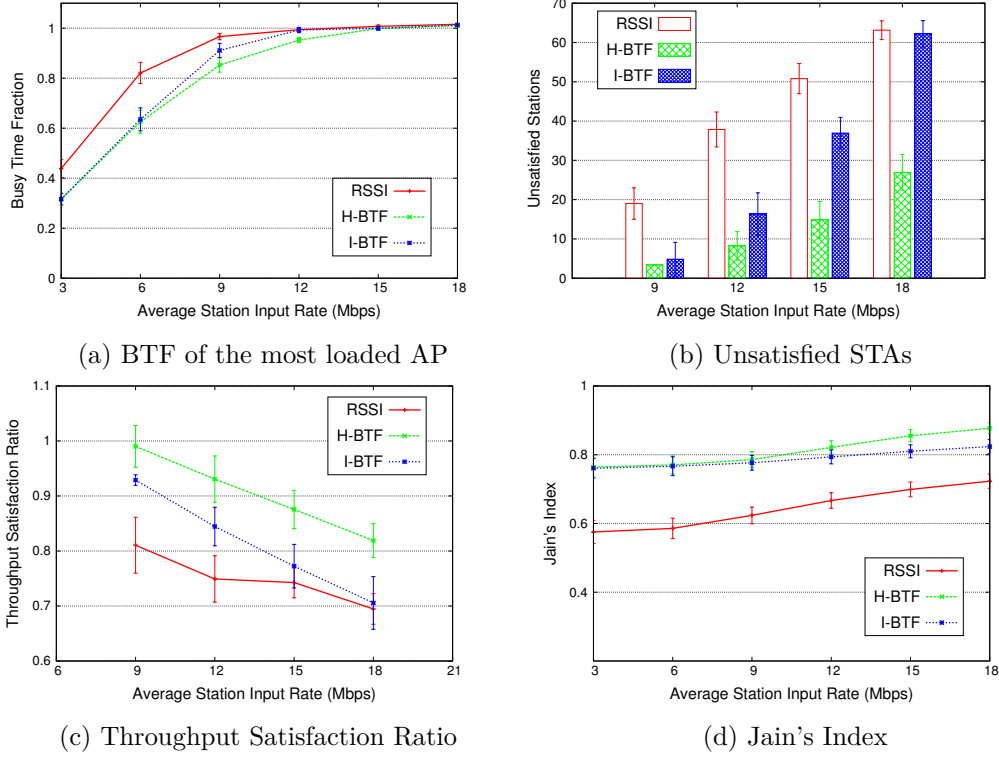
Figure 5.3: BTF association optimization using the random topology with UDP flows
