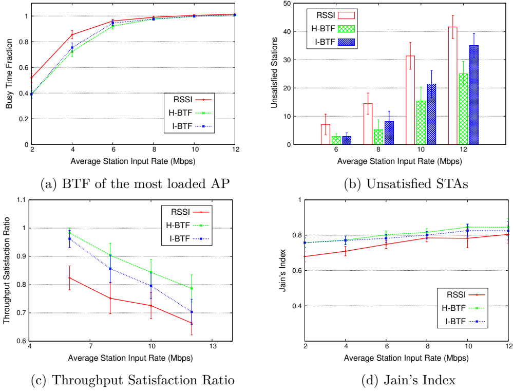
Figure 5.5: BTF association optimization using the random topology with trace flows
