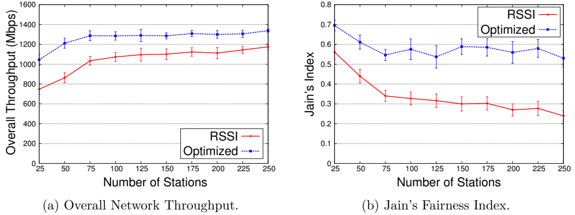
Figure 3.3: All Orthogonal channels.
