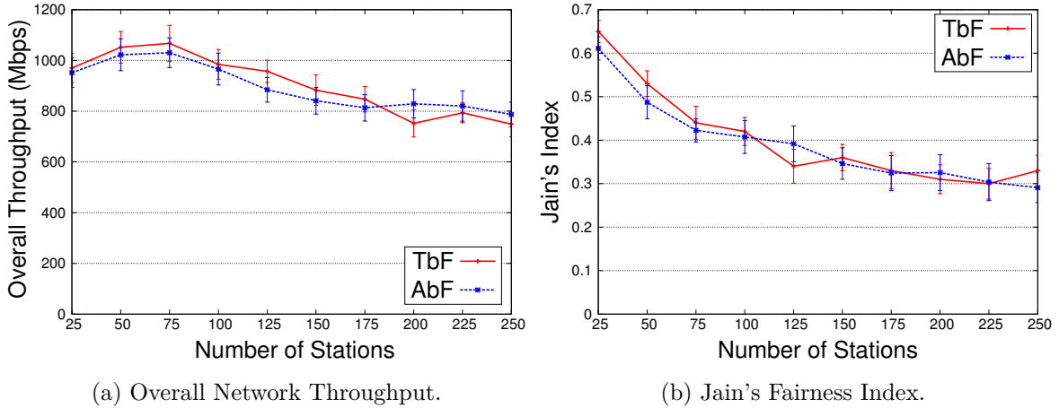
Figure 3.12: 8 Orthogonal Channels
