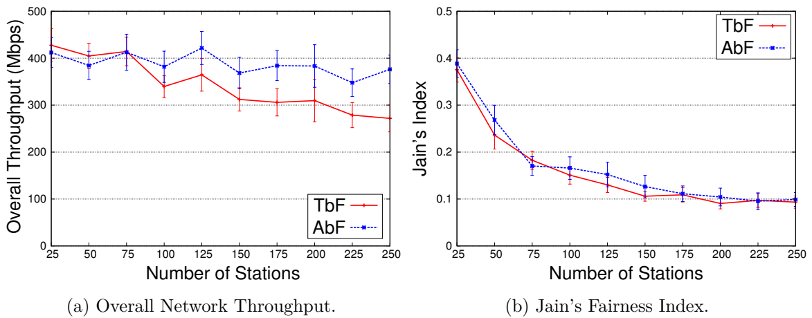
Figure 3.13: 3 Orthogonal Channels
