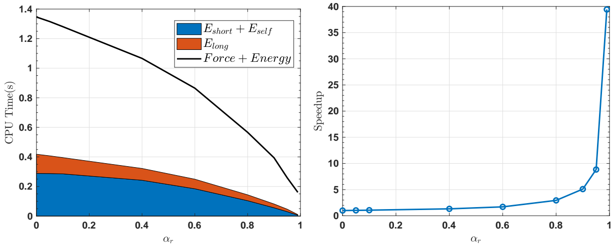
(1) Timing of the incremental evaluation of energy. The real space cost is shown in blue while the reciprocal cost is in red. The timing including incremental forces is shown as reference. (2) Speedup of the incremental evaluation of energy (only).
