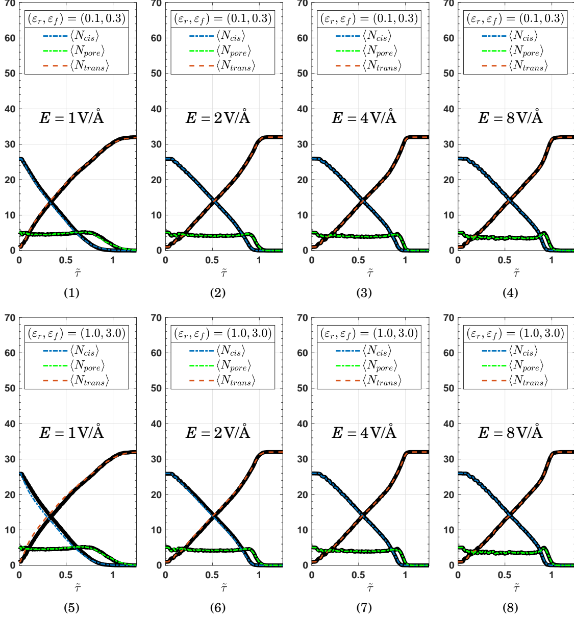
Figure 5.7: Variations of the number of monomers in the cis-region (blue), trans-region (red) and the pore (green) for the N = 32 polymer. Various configurations of restraining parameters (\varepsilon_r, \varepsilon_f) are compared. Precisely, figures (1-4) output results from simulations where (\varepsilon_r, \varepsilon_f) = (0.1, 0.3) [kcal/mol]. Analogously bottom figures (5-8) are associated to (\varepsilon_r, \varepsilon_f) = (1.0, 3.0) [kcal/mol]. The results from reference simulations (\varepsilon_r = \varepsilon_f = 0) kcal/mol are plotted with thick black solid lines and are available in figure B.2.
