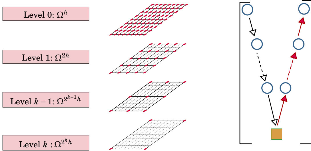
Figure 2.3: Sketch of multigrid V-cycle on a hierarchy of k + 1 grids. For each grid \Omega^{2^h} , red dots represent grid points.
