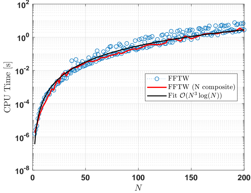
Figure 2.2: FFTW performance on various input sizes.
