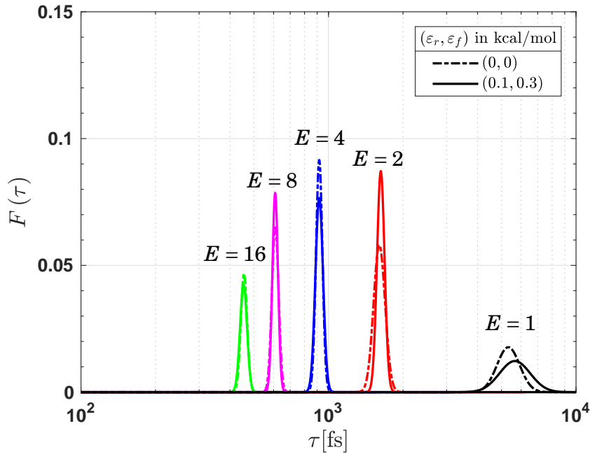
Figure 5.5: Translocation time distributions of the polymer ( N = 32 ) driven by an electric field. Two sets of restraining parameters (\varepsilon_r, \varepsilon_f) were compared. Distributions obtained with (0, 0) [kcal/mol] are displayed with dash dotted line. Results from (0.1, 0.3) [kcal/mol] simulations are shown with solid line. Various magnitudes of the electric field E were considered. A base-10 logarithmic scale is employed for the x-axis. Raw data were fitted to the time passage distribution (equation (5.8)).
