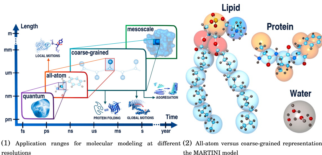
Figure 1.6: Application ranges for molecular modeling at different resolutions (Left). Sketch of the coarse-grained representation in the Martini model(right). Pictures taken from Kmiecik et al. [111]
