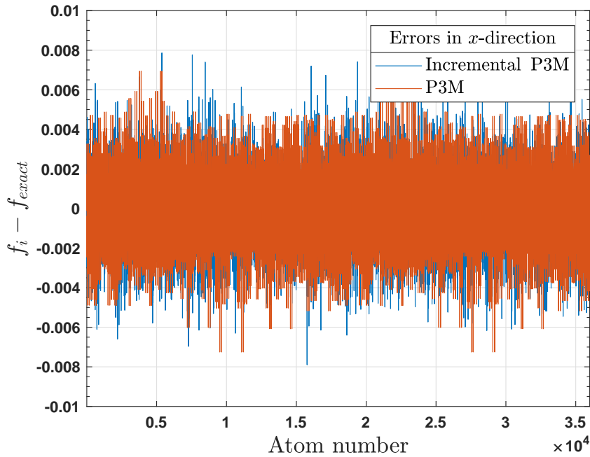
Figure 3.10: Error in forces (x-direction) of incremental P3M .
