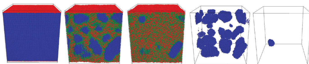
Figure 1.2: Molecular Dynamics Simulation of Laser Melting of Nanocrystalline Au. Snapshots of atomic configurations during the melting process in a 20nm nanocrystalline Au film irradiated with a 200 fs laser pulse at an absorbed fluence of 45 \text{ J}^2 \text{ m}^{-1} [122]
