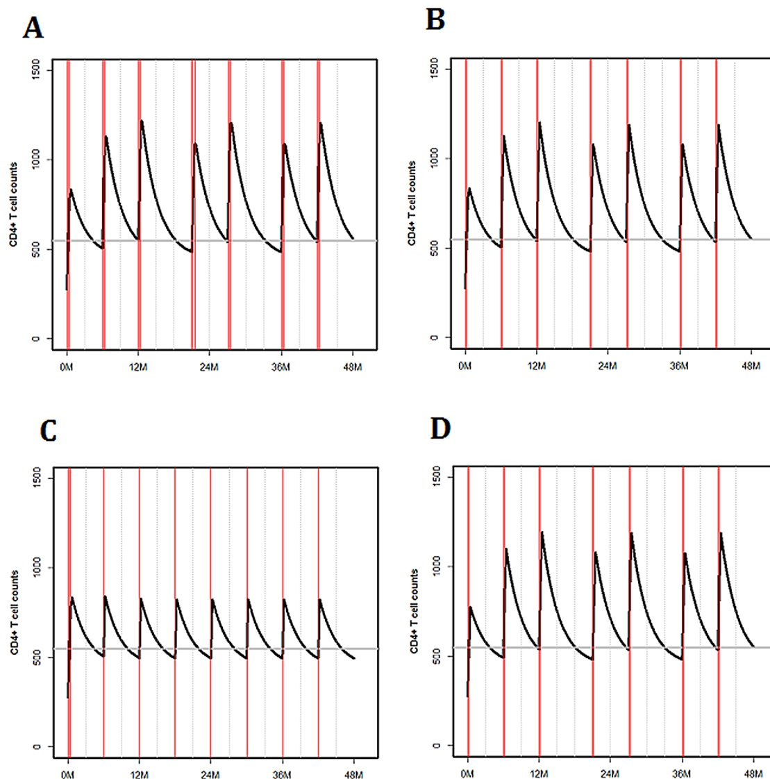
FIG. 2. CD4 count ( \text{cells}/\mu\text{L} ) predictions for 4 years for a patient having u_{\rho}^i = u_{\lambda}^i = 0 , for the four protocols A, B, C, D. Vertical dotted lines are CD4 count assessments (every three months) and vertical solid lines are injections. Horizontal line marks the CD4 threshold of 550 \text{ cells}/\mu\text{L} .
