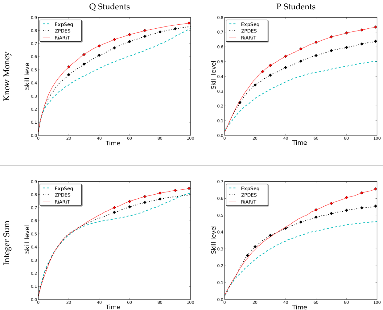
Figure 5.2: The evolution of the skill’s levels of two KC with time for population “Q” and “P”. Markers on the curve mean that the difference is statistical significant (red : RiARiT/ZPDES, black : ZPDES/ExpSeq). Both algorithms are able to improve upon the Expert Sequence.
