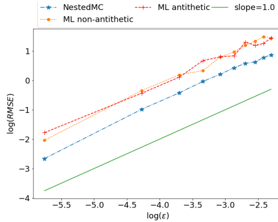
Figure 5.3: \log(\mathbf{RMSE}) w.r.t \log(\epsilon) for the butterfly option
