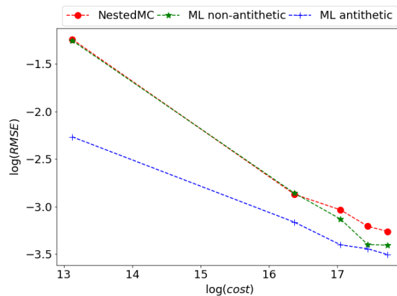
Figure 5.4: \log(\mathbf{RMSE}) w.r.t \log(\mathbf{COST}) for the butterfly option
