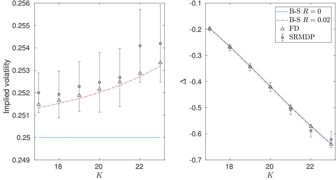
Figure 4.2: Implied volatility and delta for put options with spot value S_0 = 20 and different strikes K .
