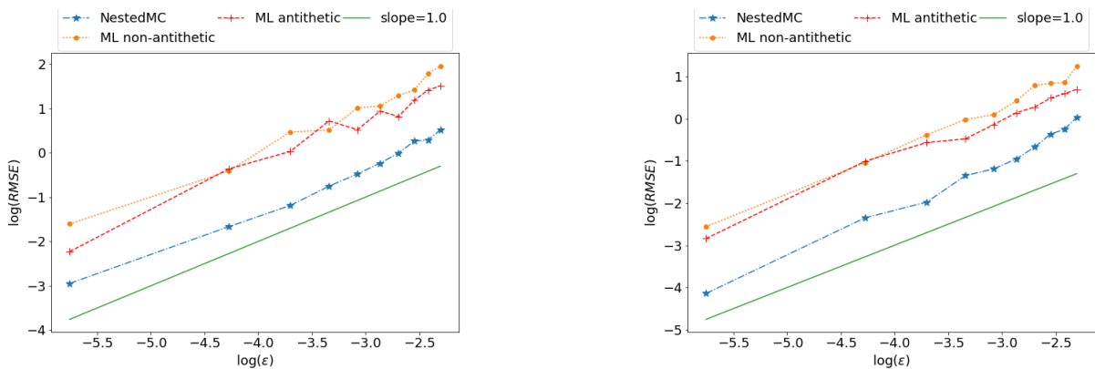
Figure 5.2: \log(\mathbf{RMSE}) w.r.t \log(\epsilon) for a call (left) and put option (right).
