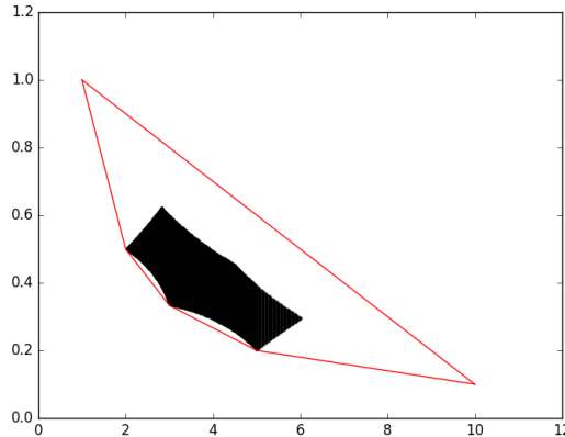
Figure 2.1: Condition (C) is satisfied for d = 5 , \lambda_1 = 1 , \lambda_2 = 2 , \lambda_3 = 3 , \lambda_4 = 5 and \lambda_5 = 10 , where n = 200 .
