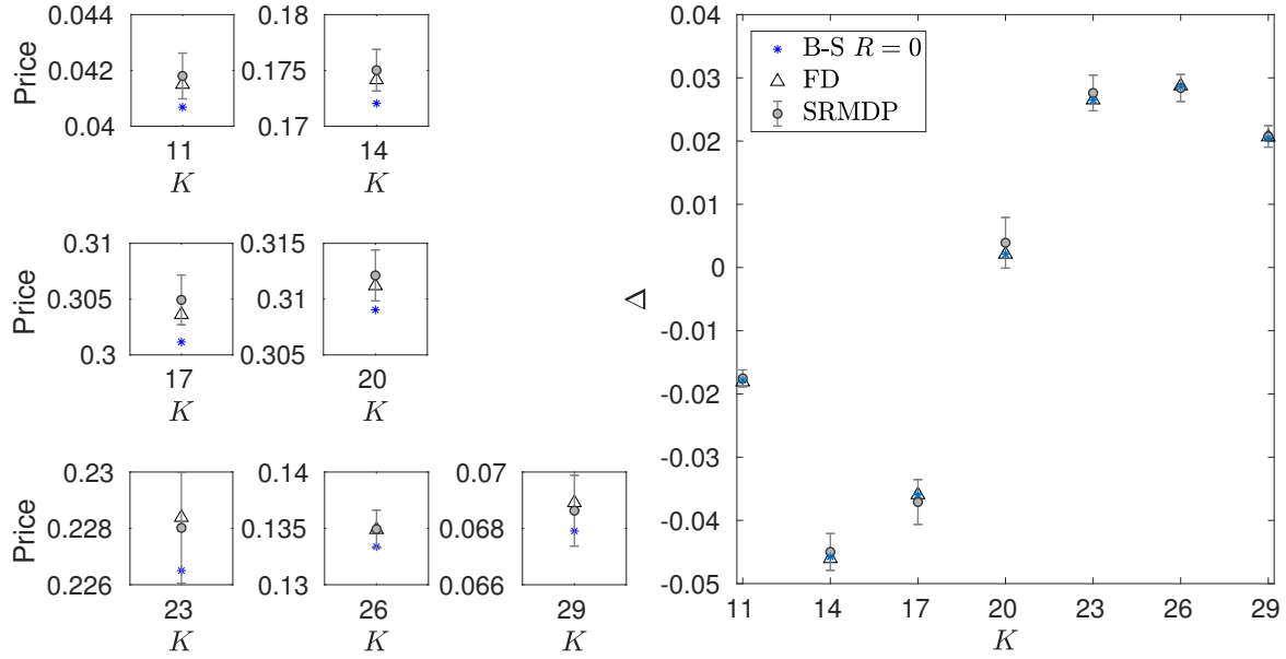
Figure 4.3: Price and delta for butterfly options with spot value S_0 = 20 and different strikes K .
