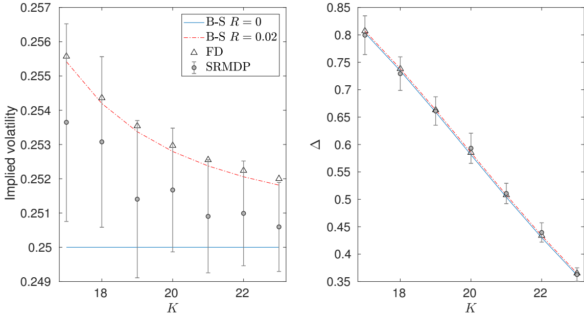
Figure 4.1: Implied volatility and delta for call options with spot value S_0 = 20 and different strikes K
