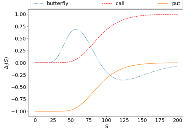
Figure 5.1: Delta for a call, put and butterfly option w.r.t spot S
