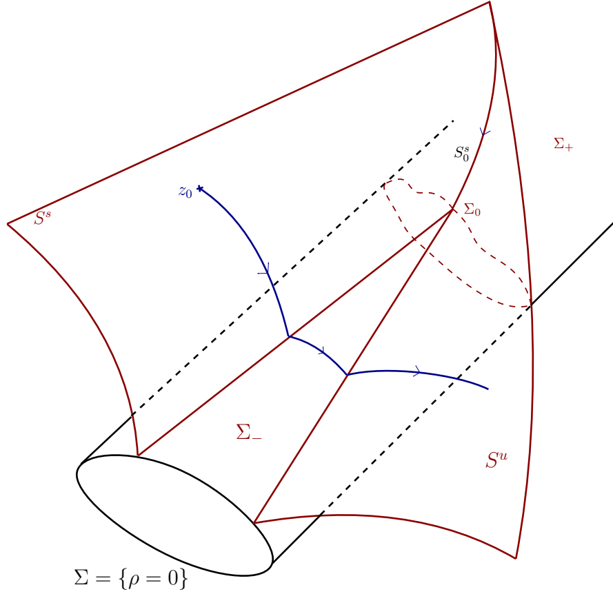
Figure 2.1: The stable and unstable manifold of \Sigma_- merging on \Sigma_0 .
