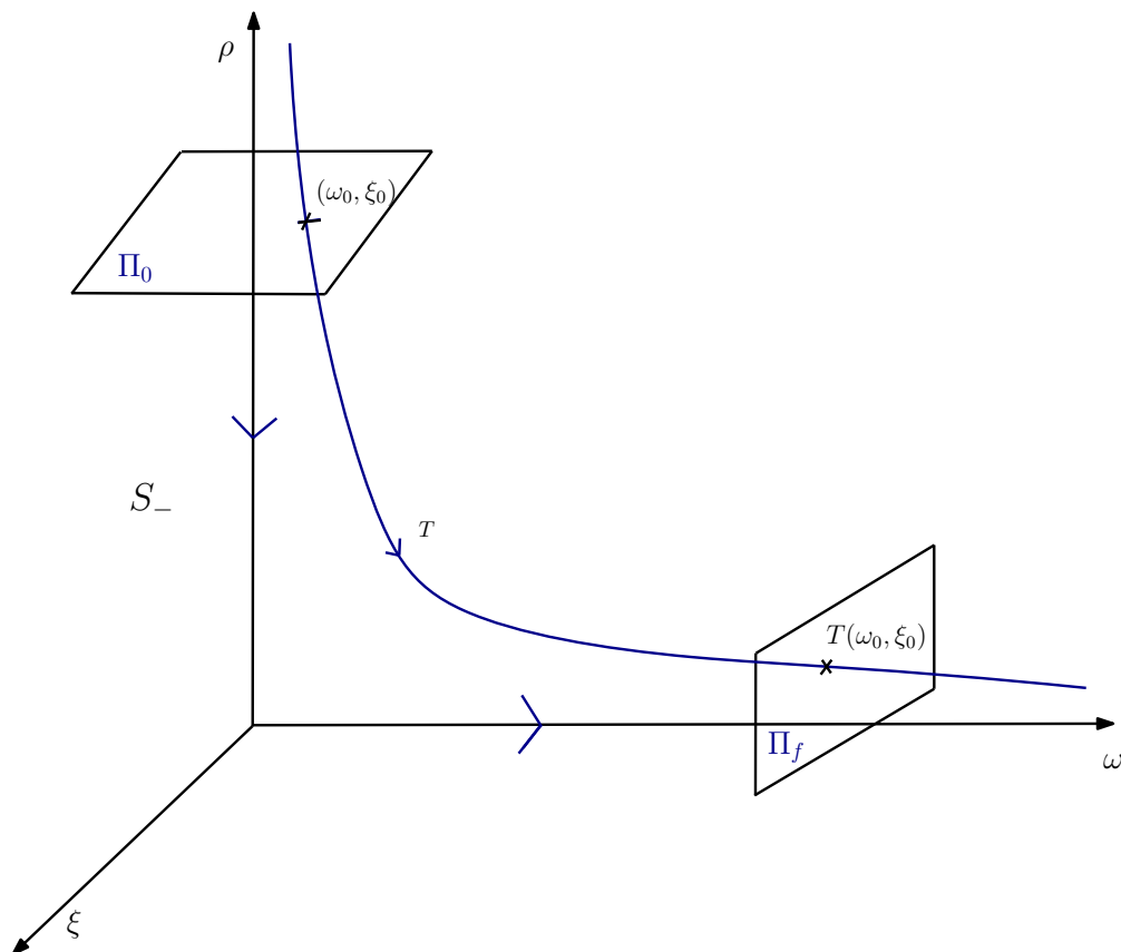
Figure 1.2: Transition map between the two sections
