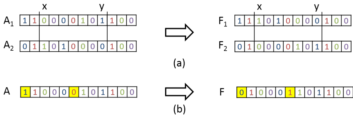
Figure 3.8: Genetic operators: a) two points crossover; b) swap mutation.
