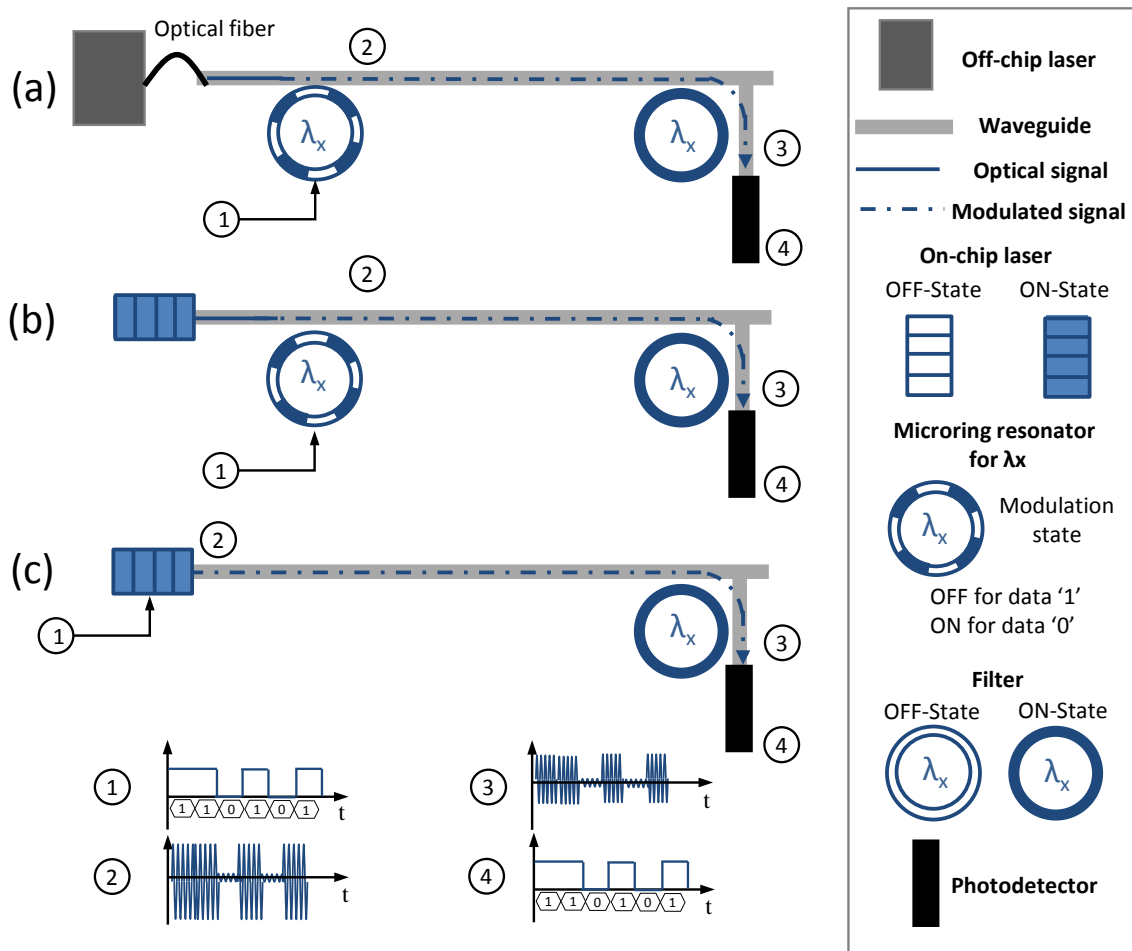
Figure 2.2: Silicon photonic interconnects with (a) external laser source using indirect modulation (b) on-chip laser using indirect modulation (c) on-chip laser using direct modulation. (1) represents the electrical signal before modulation, (2) represents the optical signal after modulation, (3) represents the optical signal before photodetection, and (4) represents the electrical signal after photodetection.
