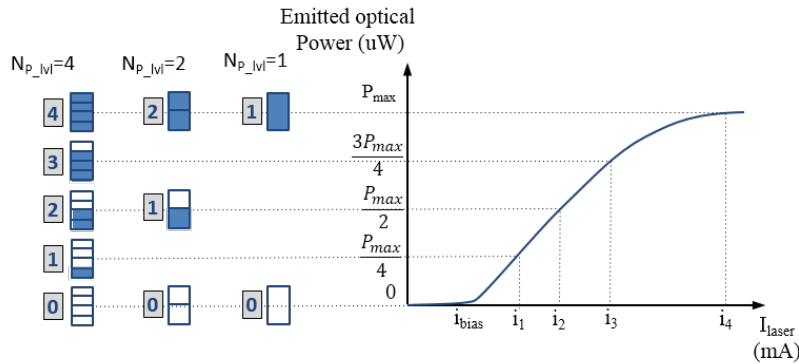
Figure 3.5: Configurable laser output power in the transmitter.
