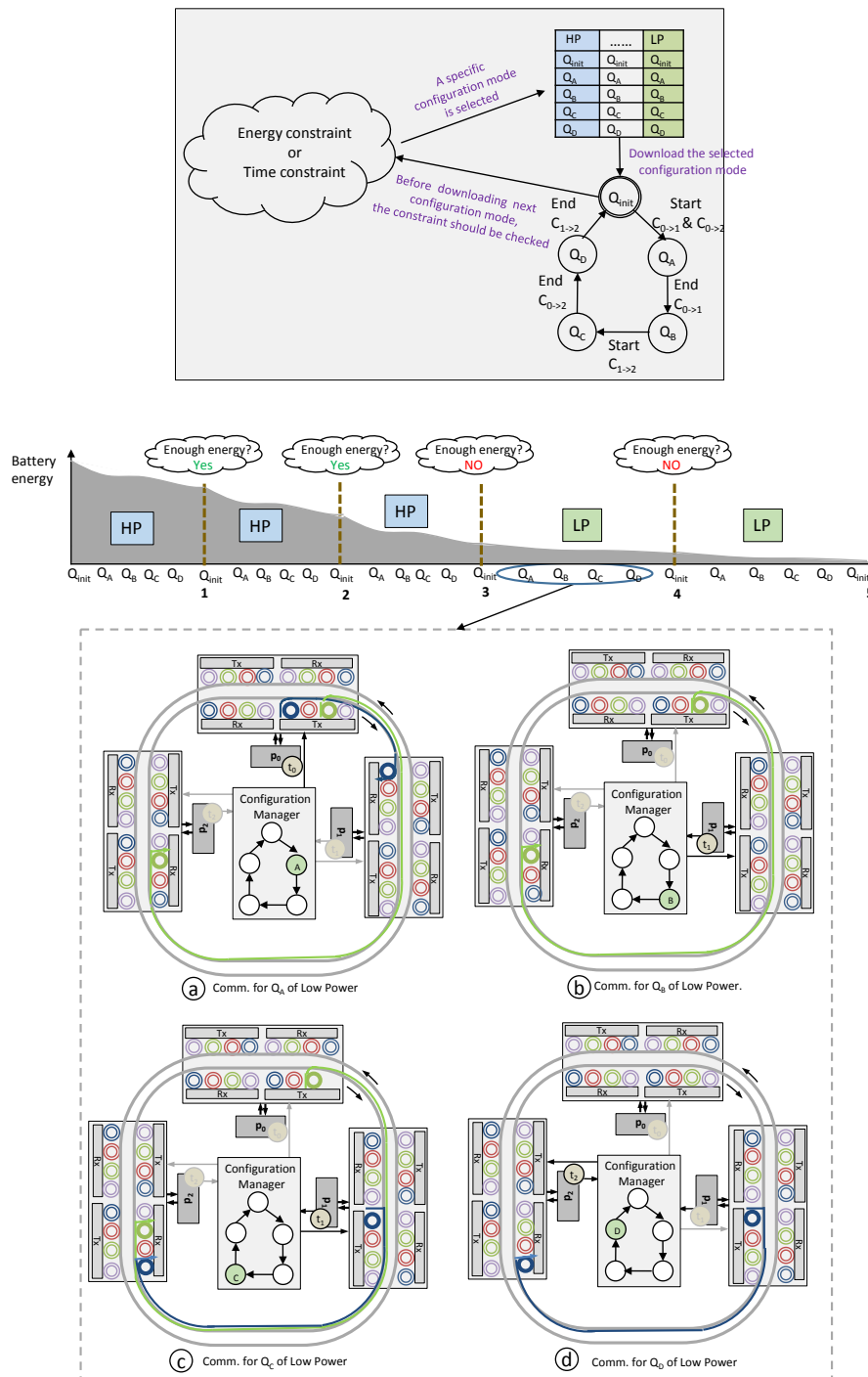
Figure 3.12: Reconfiguration of the ONoC at run-time.
