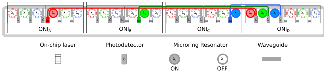
FIGURE 3.5: Multi Writer Single Reader communication scheme
