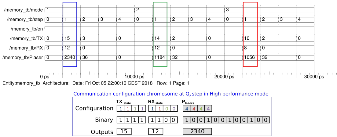
FIGURE 5.21: Manager ONI simulation result
