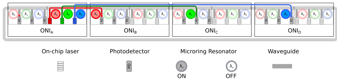
FIGURE 3.4: Single Writer Multi Reader communication scheme
