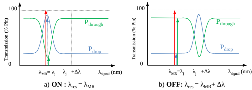
FIGURE 3.9: a) ON state and b) OFF state of MR [56]
