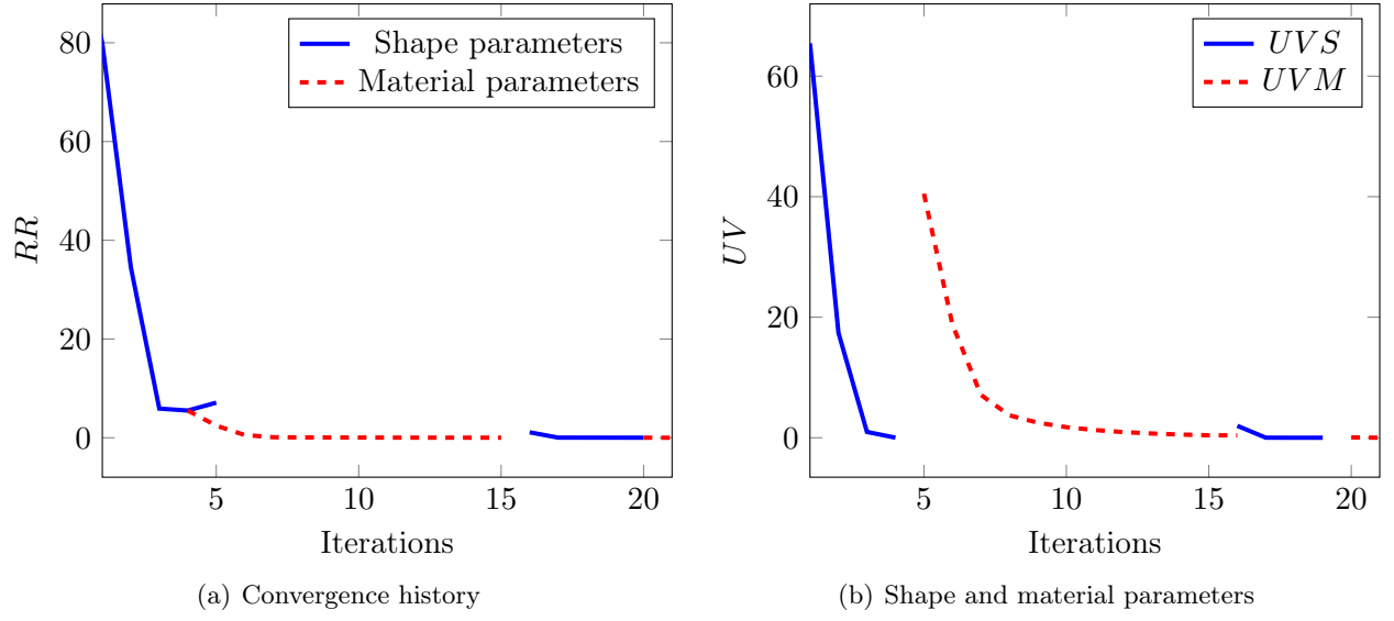
Fig. 3.4.10: Convergence history and UVS and UVM of the case of a disk shaped scatterer with a = 1\text{cm} , \lambda = 115.4\text{GPa} , \mu = 76.9\text{GPa} , \rho_s = 7900\text{kgm}^{-3} , ka = 2.67 SWRA , updated regularization parameters \alpha_m = 10^{-4} , 10^{-6} , \alpha_s = 10^{-2} , Noise level= 0%.
