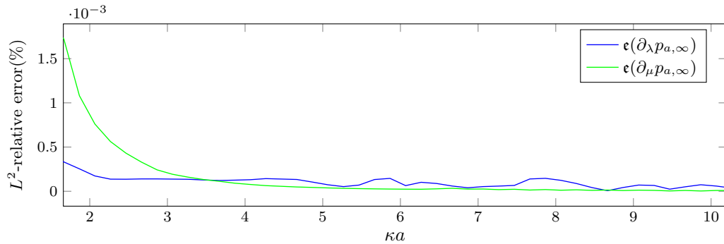
Fig. 2.2.10: Comparison between the analytical and numerical values of the Fréchet derivative of FFP, \mathfrak{e}(\partial_\lambda p_\infty) , \mathfrak{e}(\partial_\mu p_\infty) .
