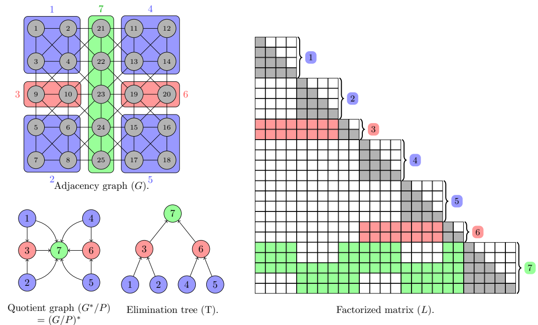
Figure 1.2: Nested dissection and block-data structure for L .
