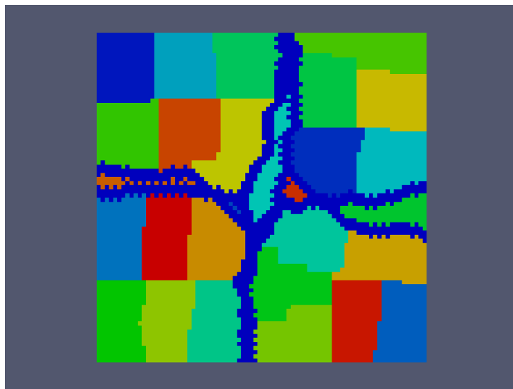
Figure 5.3: Two levels of trace for the last separator of a 80 \times 80 \times 80 Laplacian matrix.
