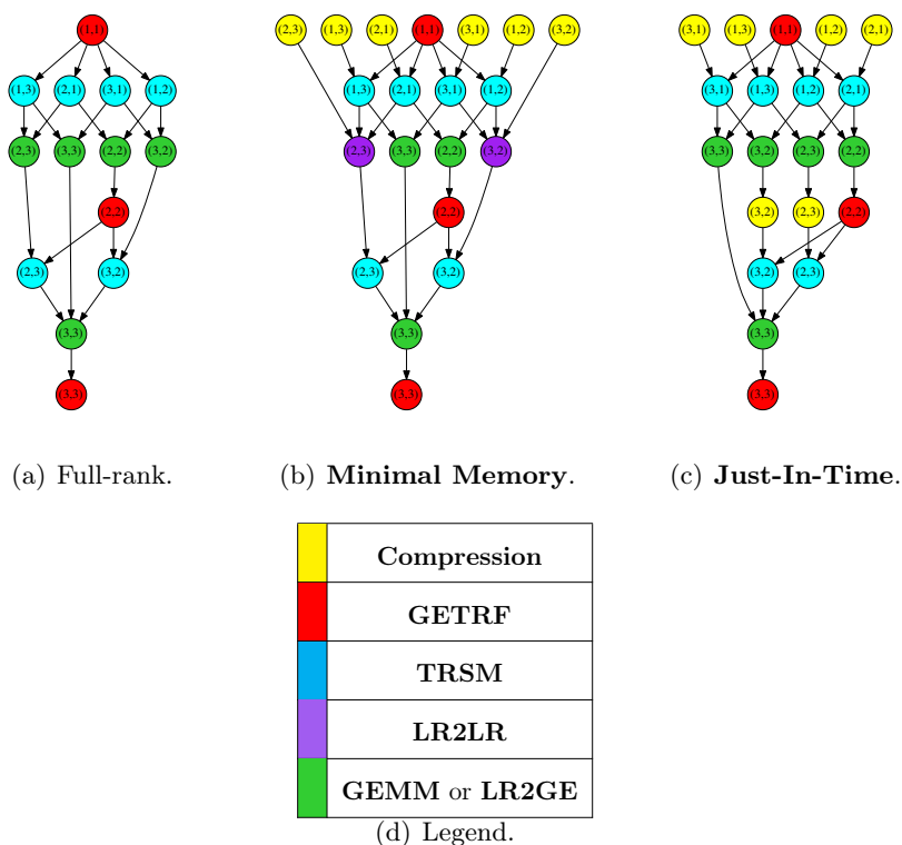
Figure 3.3: DAGs of full-rank and both low-rank strategies for the factorization of a 3-by-3 dense block matrix.
