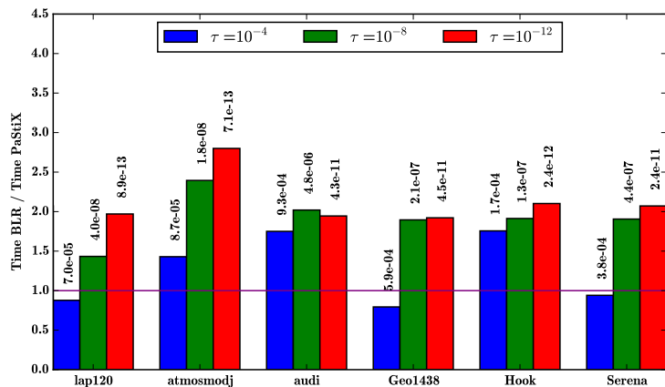
(b) Minimal Memory scenario using RRQR.
