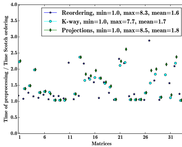
(b) Impact on preprocessing time.
