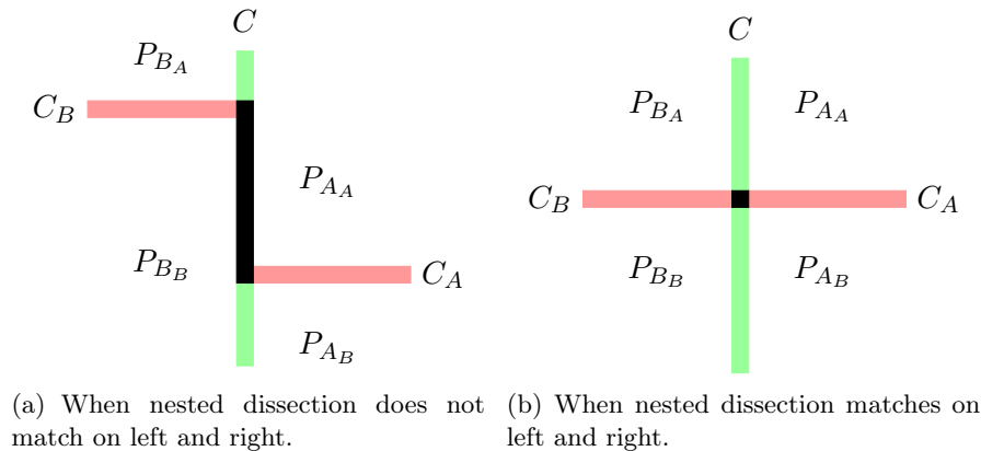
Figure 6.3: Two levels of nested dissection on a 2D graph. On the left, non-aligned separators are illustrated, which increases the sets of possible contributions on C . On the right, separators are aligned, which reduces the number of combinations of contributions on C .
