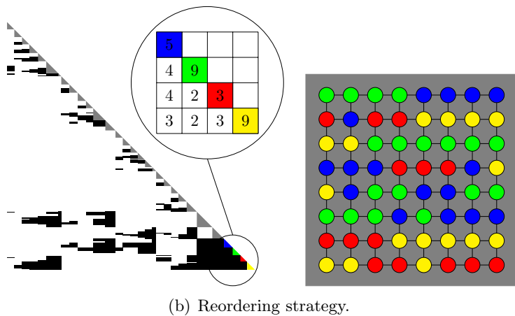
Figure 5.1: Illustration of the clustering obtained through the k-way partitioning, on top, and the reordering heuristic, on bottom, for the top-level separator of size 8 \times 8 of a 8 \times 8 \times 8 regular grid. The symbolic factorizations, on the left, show the evolution of the off-diagonal blocks in number and size with a focus on the number of external contributions applied to each block of the matrix associated with the last separator ( A_{22} ). The meshes, on the right, show the distribution of the unknowns into the clusters on the graph of the separators.
