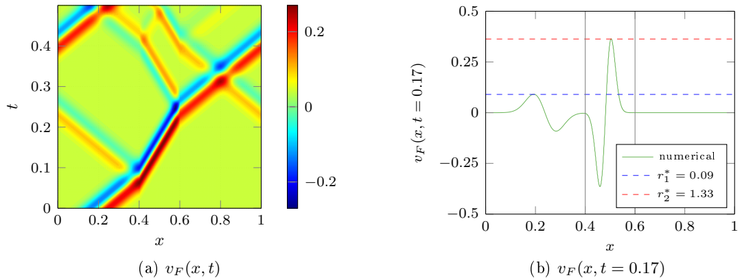
FIGURE 6.13: Propagation of the numerical velocity v_F(x, t) in a heterogeneous 1D fluid domain.
