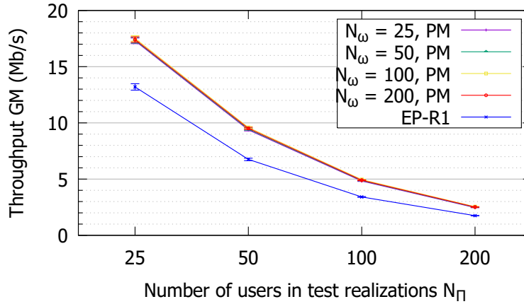
Figure 3.8: Throughput geometric mean function of the number of users in test realizations N_\pi , for different values of the number of users in calibration realizations N_\omega , for b = 5 sub-bands, and |\pi| = 100 test realizations.
