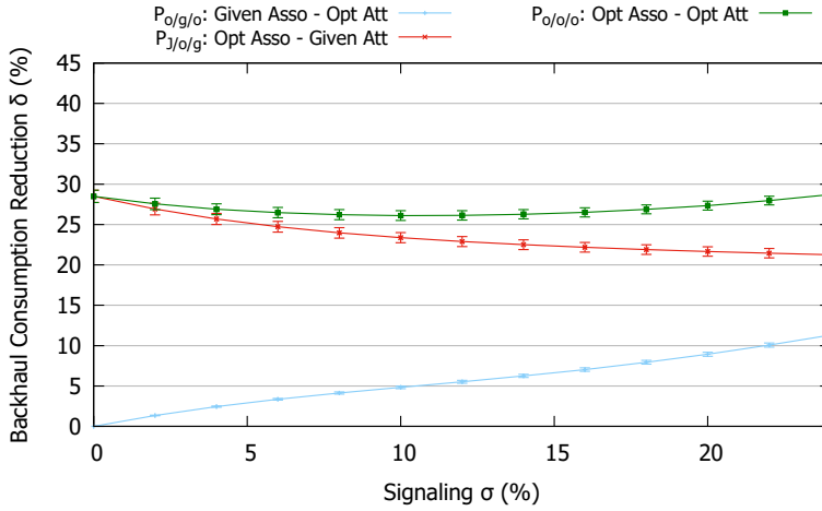
Figure 5.8: The relative backhaul bandwidth consumption reduction \delta function of \sigma , in \mathcal{P}_{o/g/o} , \mathcal{P}_{\mathcal{J}/o/g} , and \mathcal{P}_{o/o/o} .
