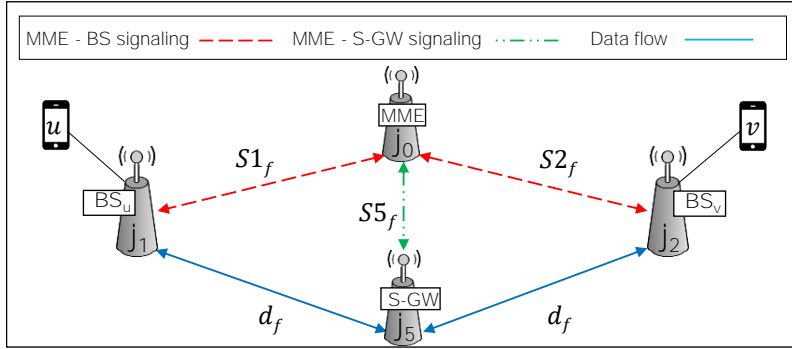
Figure 5.2: Data and signaling traffic paths between BSs, and their corresponding bit rates d_f and S_{i_f} , for a flow f , when there is one S-GW in the network ( \mathcal{P}_{1/g/g} ), or when attachment is optimized per flow ( \mathcal{P}_{o/g/of} , and \mathcal{P}_{o/o/of} )
