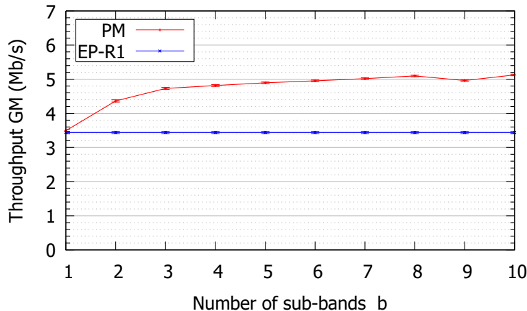
Figure 3.6: Throughput geometric mean function of the number of sub-bands b , tested on |\pi| = 100 test realizations, with N_\pi = 100 users in each test realization, with a power map obtained for |\Omega| = 10 calibration realizations, and N_\omega = 100 users.
