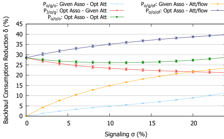
Figure 5.10: The relative backhaul bandwidth consumption reduction \delta function of \sigma , in \mathcal{P}_{o/g/o} , \mathcal{P}_{o/g/of} , \mathcal{P}_{o/o/o} , \mathcal{P}_{o/o/of} , and \mathcal{P}_{o/o/g} .
