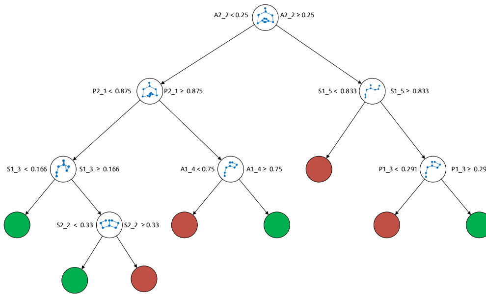
Figure 6.15: Ground-Truth
