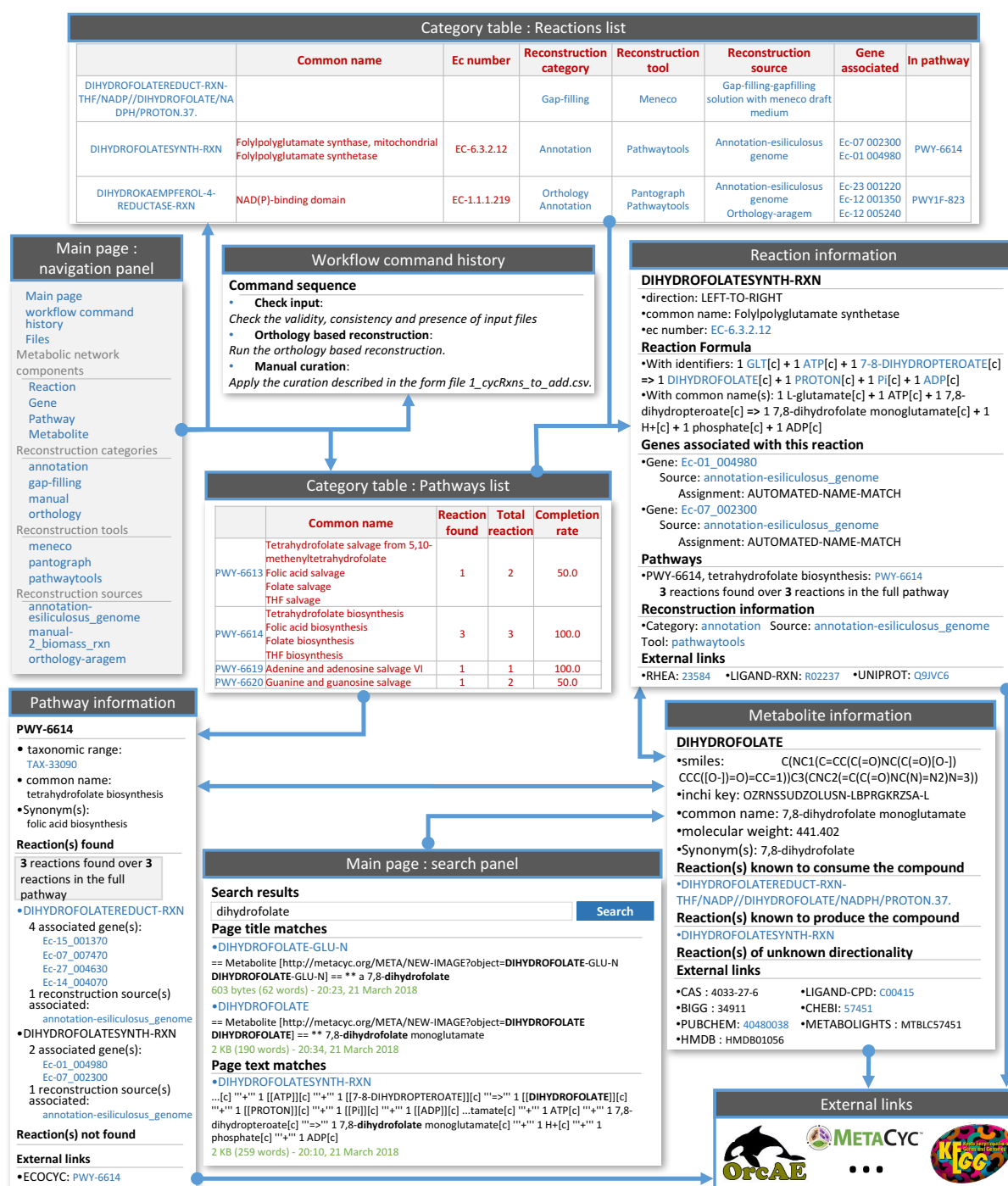
Figure 7.1: Screen captures of several pages of the local wiki and the interactions between them
