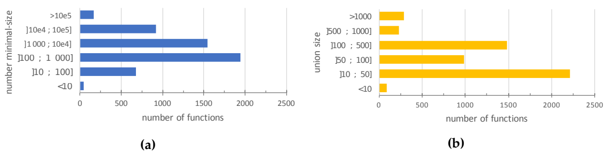
Figure 5.7: Enumeration and union of minimal-size solutions
