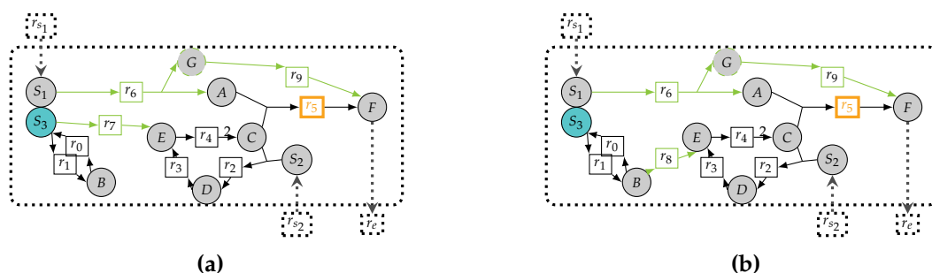
Figure 3.6: Solutions to hybrid metabolic network completion
