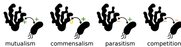
Figure 1.2: Classical ecological pairwise interactions
