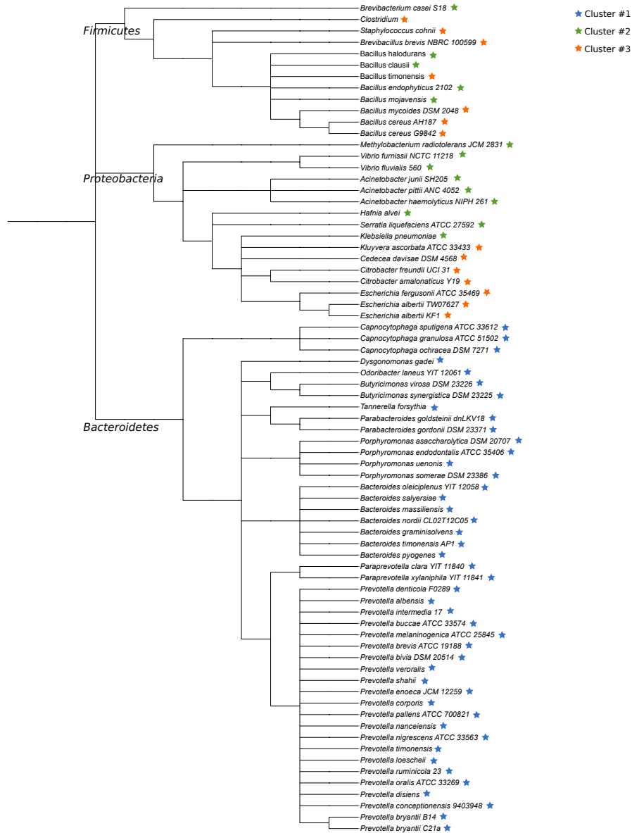
Figure B.1: Taxonomic tree of the 89 gut bacteria
