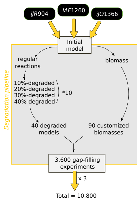
Figure 2.1: Degradation pipeline of E. coli GSMs
