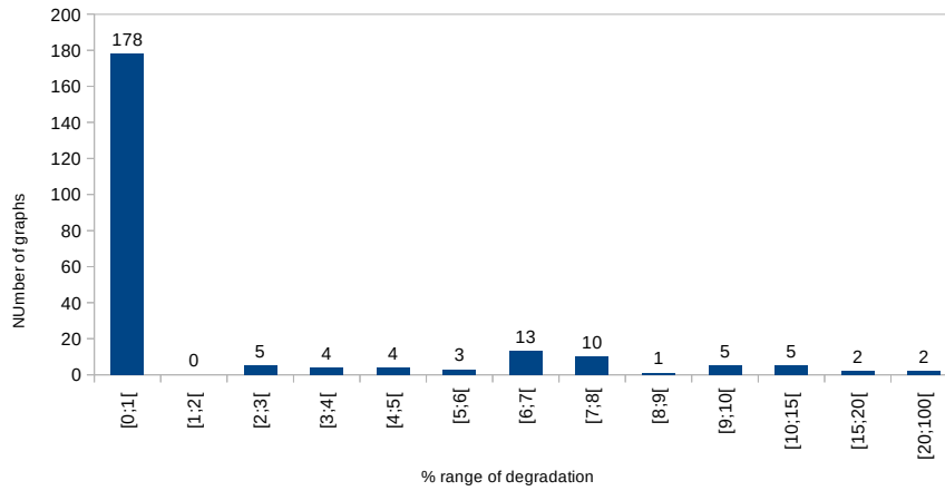
Figure 4.5 – Distribution degradation heuristic vs ILP (232 test-cases)
