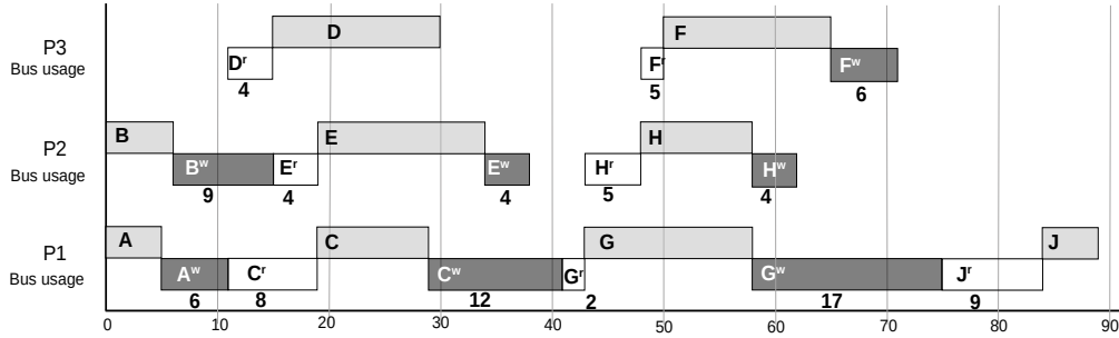
(b) Resulting schedule with a contention-aware contention scenario – overall makespan is 89 time units.
