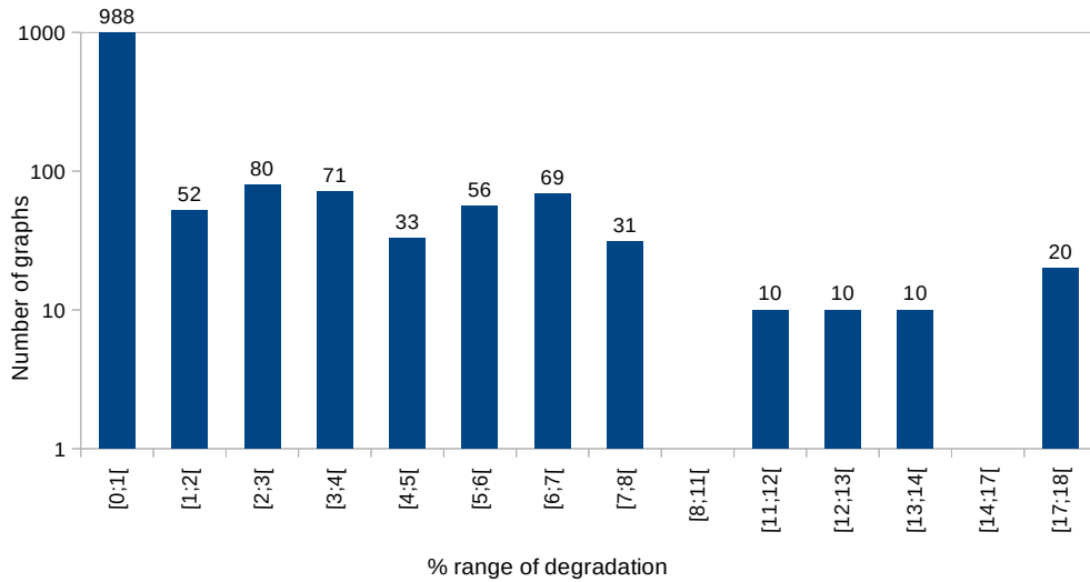
Figure 2.6 – Distribution of the degradation of the heuristic against the ILP formulation using STG task set. (logarithmic scale)
