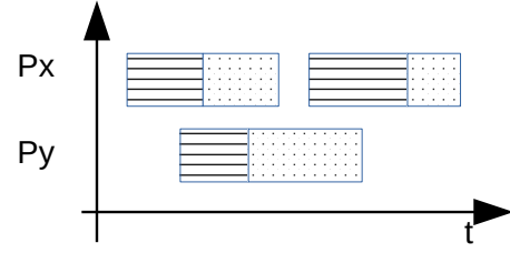
(b) Example of three tasks using PREM, a memory phase accesses the off-chip memory to write or read data, then the execute phase can compute without any more accesses to the shared memory.
