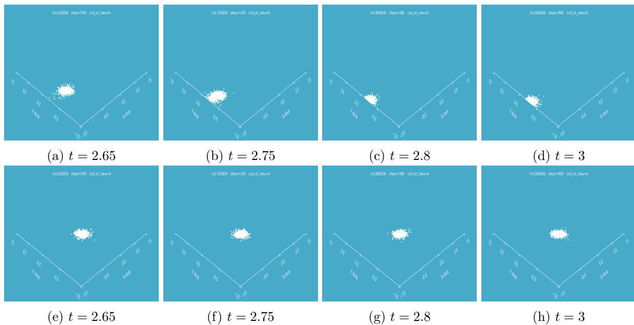
Figure 7.4: The continuation of the evolution in Figure 7.3–(a)-(e): PDDM; (f)-(j): PPPM.
