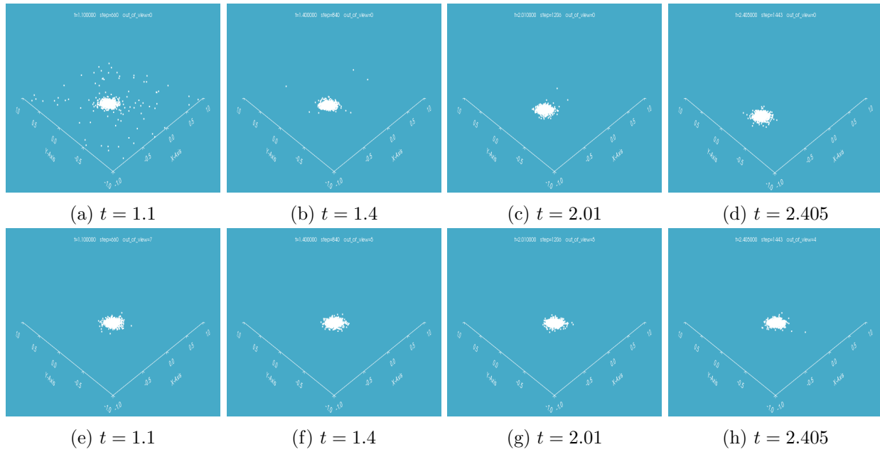
Figure 7.3: The continuation of the evolution in Figure 7.2–(a)-(e): PDDM; (f)-(j): PPPM.
