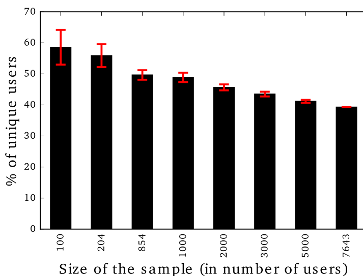
Figure 7.13 – Uniqueness of Chrome users based on their extensions only vs. number of users - 204 is the number of users used in [245] and 854 the number of users considered in [260]
