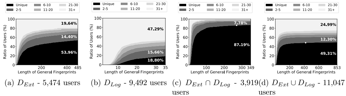
Figure 7.11 – Anonymity sets for different numbers of attributes tested by general fingerprinting algorithm.
