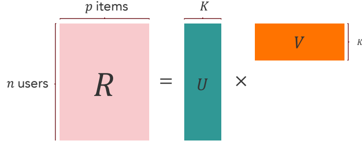
Figure 3.2: Matrix Factorization.
