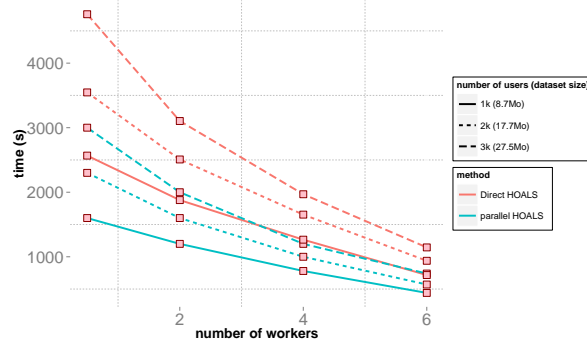
Figure 3.5: Result of the scalability test of parallel HOALS ran with the implicit version with rank constraints of 200 for users and items and 2 for actions. Each workers has 2CPUs.
