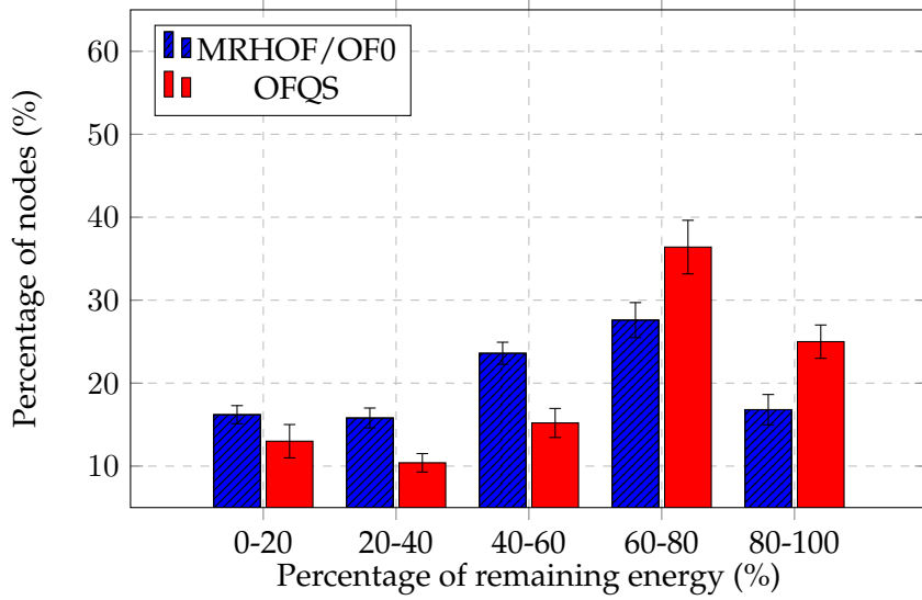
FIGURE 3.12: Remaining energy distribution among the nodes after 30 minutes
