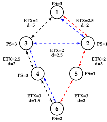
FIGURE 3.2: Network with different ETX , delay d (in ms) and PS values
