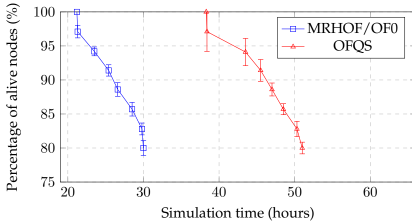
FIGURE 3.4: Network lifetime variation
