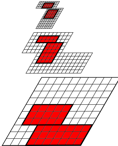
Figure 1.4: Telescopic representation of the block-structured adaptive mesh refinement. In red are highlighted the parts of each telescopic level, partially refined in the next step, just on the surface concerned by the refining. The refined portions can be chosen using, for example, the Berger–Colella algorithm
