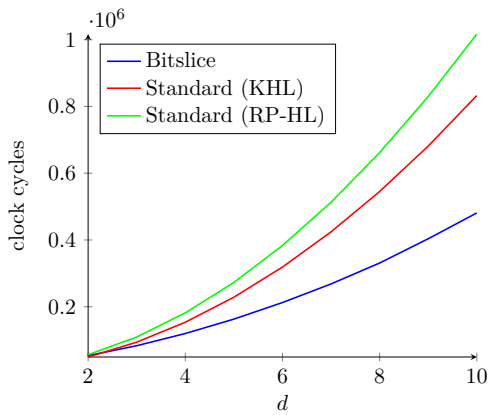
Figure 5.14: Timings of masked AES.
