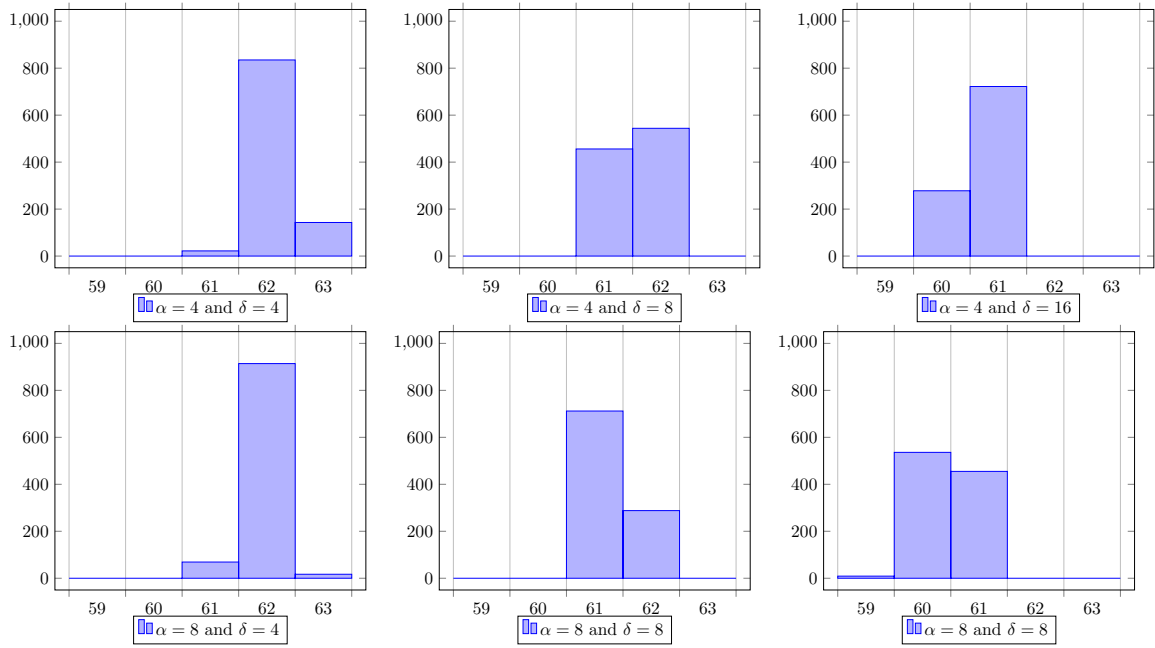
Figure 3.2: Number of Random S-boxes for each Multiplicative Complexity for n = 8
