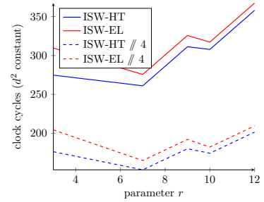
Figure 3.5: CRV d^2 const. ( \lambda = 8 ).
