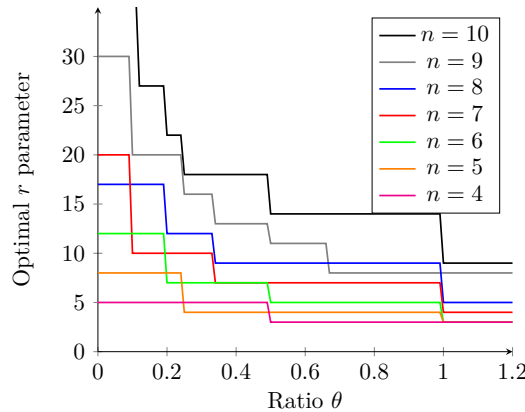
Figure 3.3: Optimal r parameter w.r.t. the CPRR-ISW cost ratio \theta for \lambda \in \llbracket 4, 8 \rrbracket .
