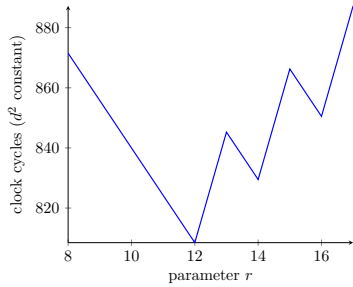
Figure 3.4: CRV d^2 const. ( \lambda = 6 ).
