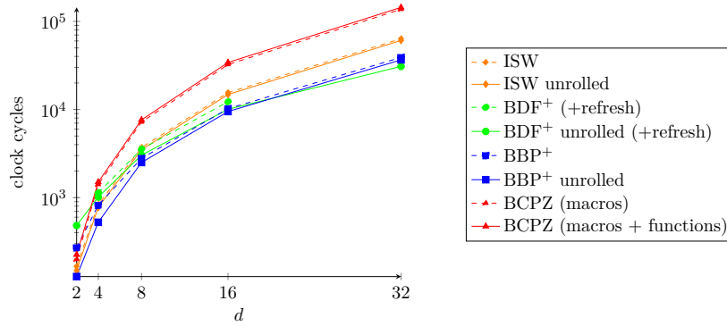
Figure 5.4: Multiplication performances for TRNG-2 in clock cycles
