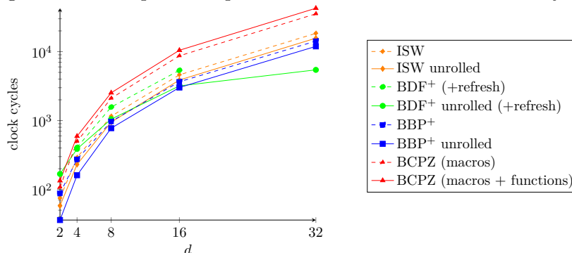
Figure 5.3: Multiplication performances for TRNG-1 in clock cycles
