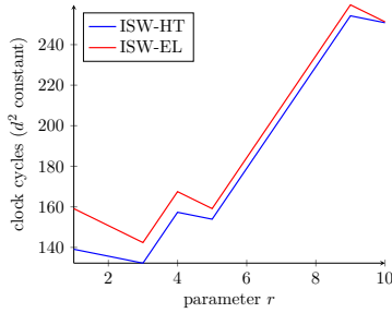
Figure 3.4: CRV d^2 const. ( \lambda = 6 ).
