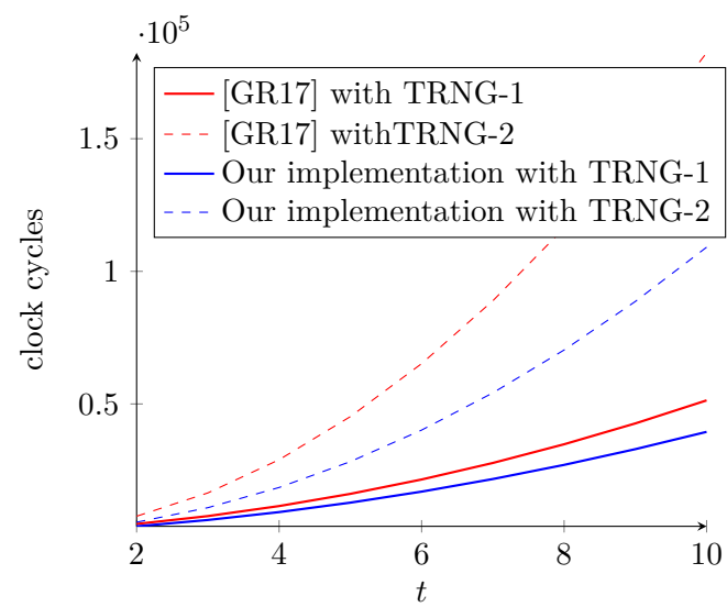
Figure 4.15: Timings of a t -probing secure AES s-box implementation.
