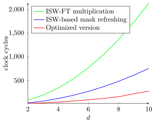
Figure 5.2: Timings of mask refreshing.
