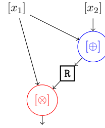
Figure 4.2: Graph representation of Circuit 1 after maskComp .
