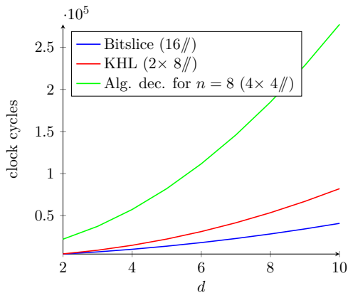
Figure 5.12: Timings for 16 AES s-boxes.
