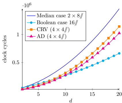
Figure 5.8: Timings for n = 8 .
