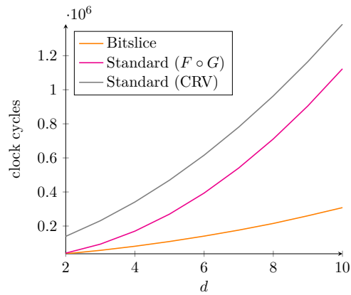
Figure 5.15: Timings of masked PRESENT.
