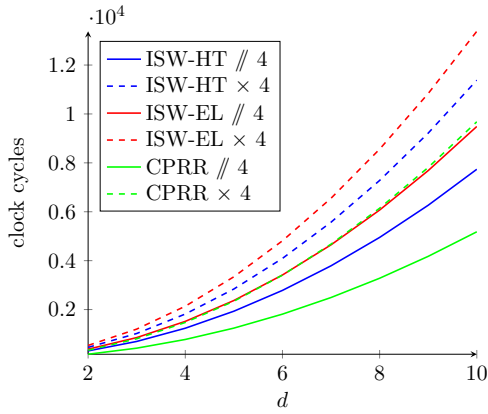
Figure 5.6: Timings of (parallel) ISW and CPRR schemes for n = 8 .
