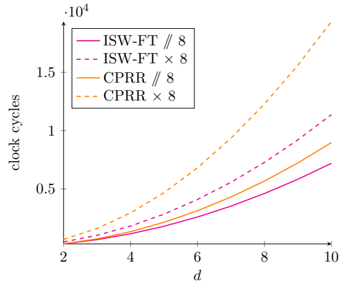
Figure 5.7: Timings of (parallel) ISW and CPRR schemes for n = 4 .
