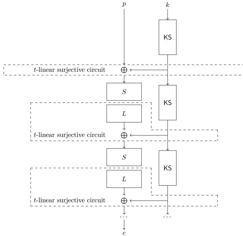
Figure 4.11: Structure of an SPN-Based Block Cipher.
