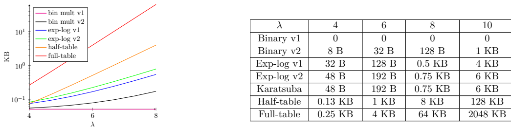
Figure 5.1: Full code size (left graph) and LUT size (right table) w.r.t. \lambda .
