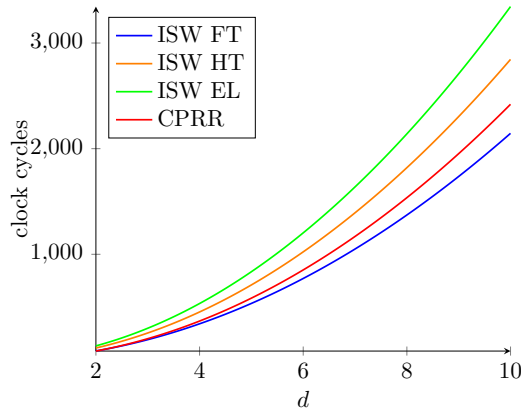
Figure 5.5: Timings of ISW and CPRR schemes.
