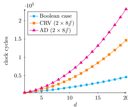
Figure 5.9: Timings for n = 4 .
