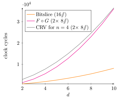
Figure 5.13: Timings for 16 PRESENT s-boxes.
