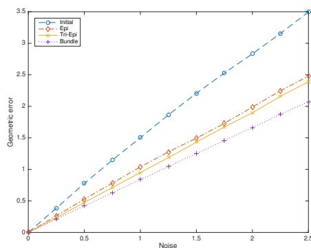
Figure 1.13: Non-collinear pinholes: quantitative results using synthetic datasets (20 points) with different amounts of Gaussian noise, in terms of the geometric distance error. The different lines represent the error of the initial approximation (Initial), and the errors of the solution refined using the trinocular-epipolar (Tri-Epi), epipolar (Epi) and bundle adjustment (Bundle) approach. The results are averages of 50 configurations of points and cameras.
