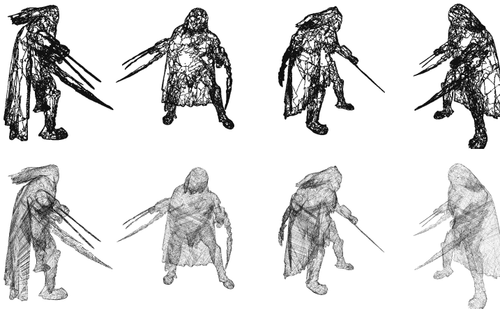
Figure 4.26: “Predator” dataset: 24 silhouettes and projection matrices. Top : Four views of the intersection curves. Bottom : Four views of a point cloud on the visual hull surface (approximately 130000 points).
