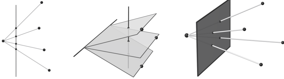
Figure 1.2: Linear projections \mathbb{P}^2 \dashrightarrow \mathbb{P}^1 (left), \mathbb{P}^3 \dashrightarrow \mathbb{P}^1 (center), and \mathbb{P}^3 \dashrightarrow \mathbb{P}^2 (right). Note that the “retinal space” is a line in the first two cases (shown in dark).
