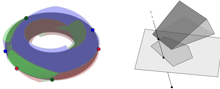
Figure 4.9: Tangential points are the intersections of a silhouette T_i with the boundary of P_i \left( \bigcap_{j \neq i} C_j \right) . Left : the silhouette of a torus and the reprojection of the visual hull generated by three different views. The six tangential points are epipolar tangencies (colors indicate projections of cone surfaces and the associated epipolar tangency points). Right : a tangential point may also be the projection of a “tangential triple point”: in this case, the associated viewing ray is not tangent to any visual cone.
